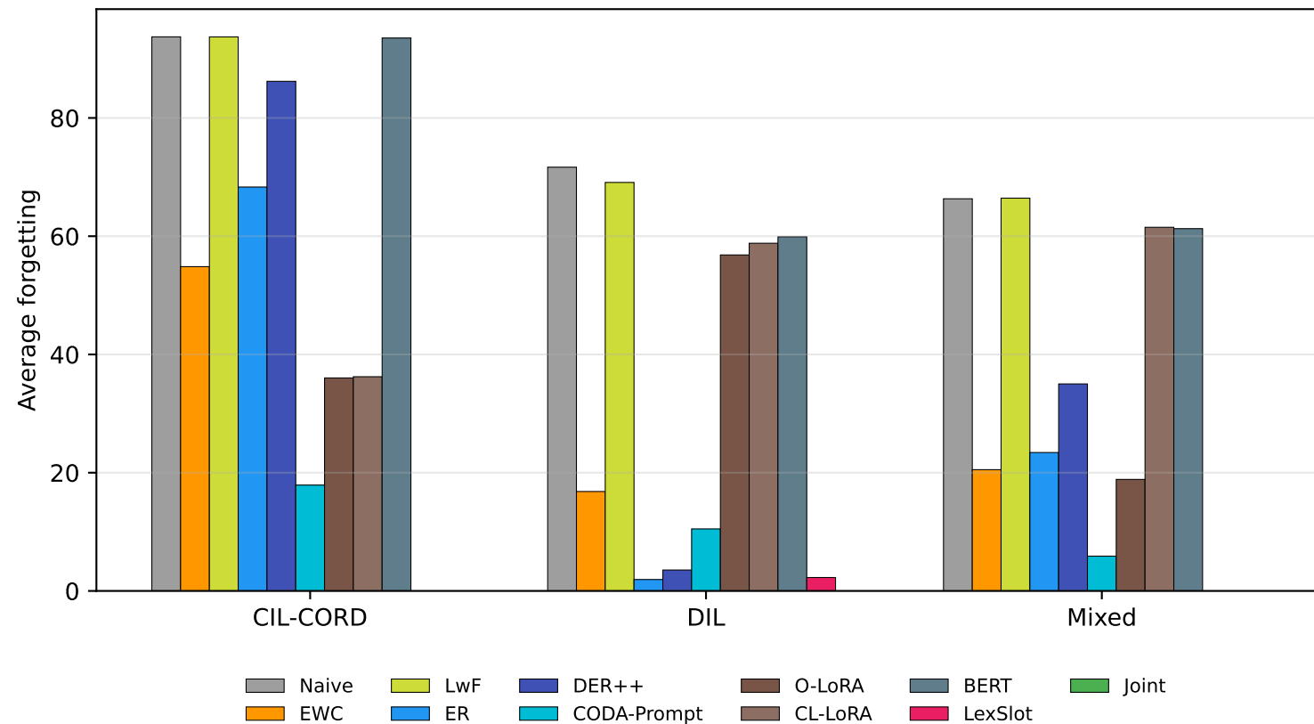
Average forgetting by method and scenario
