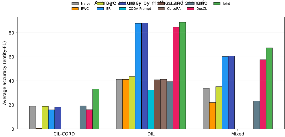
Figure 6.5: Average accuracy (AA) of each method on the three scenarios, grouped by scenario, with the naive lower bound and the joint upper bound for reference. Both replay methods (ER, DER++) reach the joint ceiling on DIL; the measured DocCL closes most of the DIL gap (84.7 vs the oracle’s 88.7, \sim 4 points short) but sits \sim 3 points below replay there and below both on Mixed (Table 6.6).
