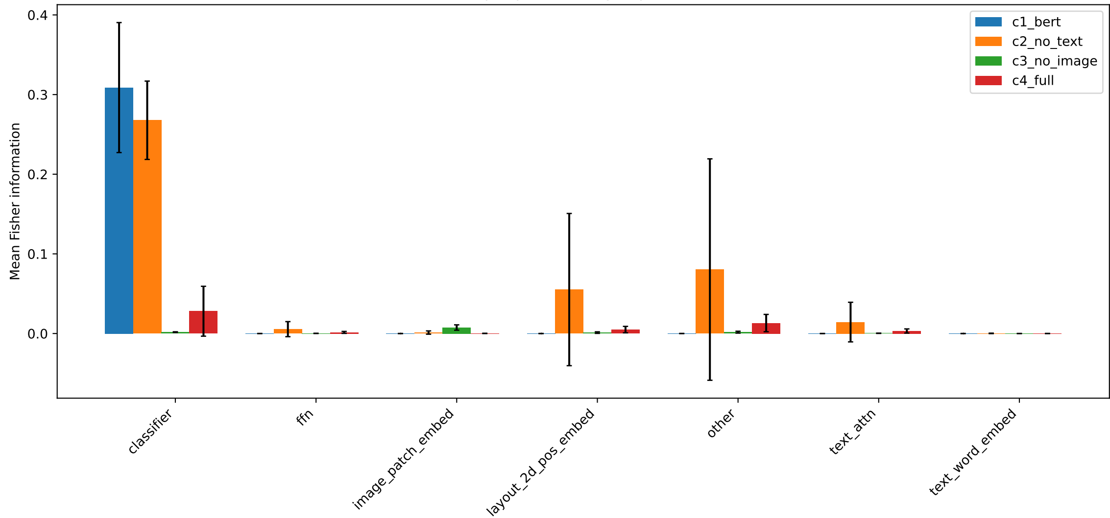
Fisher information per parameter group (after final task t=2.0)
