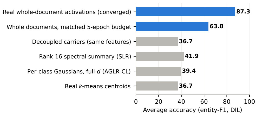
Figure 6.15: The latent-replay elimination ladder at a fixed frozen boundary (layer k=8 , DIL). Only whole-document replay (blue) retains accuracy; every summarised representation, including real k -means centroids, collapses to the naive level, and the matched-budget single-variable control (whole documents 63.8 vs. the same features on decoupled carriers 36.7) isolates whole-document (feature, position, label) binding as the necessary ingredient. Single-seed diagnostic runs (seed 42).
