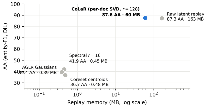
Figure 6.16: Replay memory versus retention (DIL, log-scale memory axis). CoLaR (blue) matches raw latent replay’s accuracy at 2.7\times less storage because its per-document SVD factors preserve whole-document binding; the aggressive compressions at \sim 0.4 MB all break that binding and collapse. Memory figures are serialized replay-store bytes as instrumented per run.
