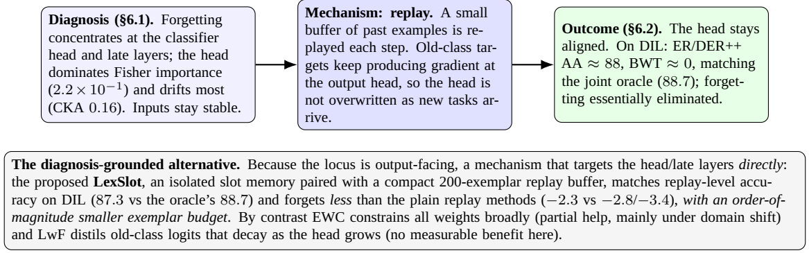
Figure 6.17: From diagnosis to result: because forgetting is output-facing, replay’s re-exposure of old-class targets keeps the classifier head aligned, which explains its empirical win (both ER and DER++ reach DIL BWT \approx 0 ). The diagnosis-grounded method, LexSlot, an isolated slot memory at the head/late layers, approaches the oracle and replay on the DIL forgetting gap (87.3 vs the oracle’s 88.7), forgets less than the plain replay methods, and does so with a compact 200-exemplar buffer (frozen backbone, an order-of-magnitude smaller exemplar budget than plain replay).
