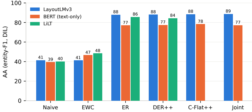
Figure 6.13: The replay-dominant ordering on DIL across backbones (mean over three seeds, from the aggregated run table). The three-tier structure (replay near the joint oracle, regularisation barely above the naive floor) reproduces on the text-only BERT backbone at a uniformly lower level and on LiLT where cells exist; C-Flat++ and Joint are not yet run on LiLT.
