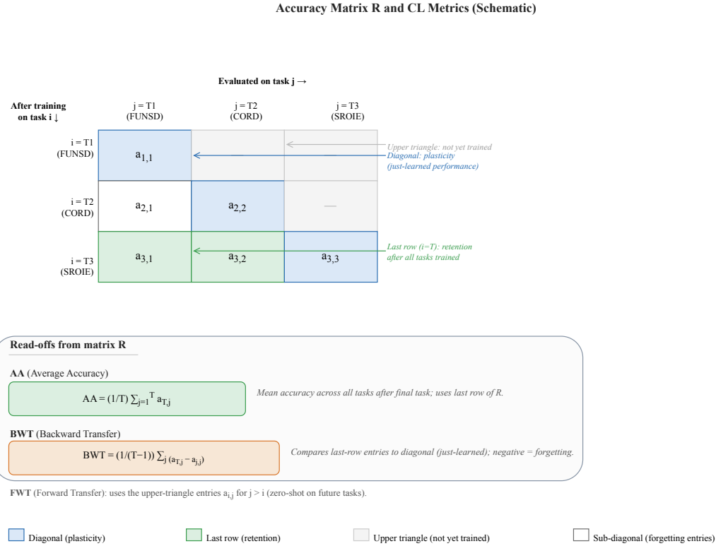
Figure 3.2: Schematic structure of the accuracy matrix R[i, j] (entity-F1 on task j after training task i ); symbolic labels only, with no measured values. The diagonal R[i, i] records just-learned accuracy; the lower triangle R[i, j] for j < i records retained accuracy on earlier tasks, from which average accuracy, backward transfer, and average forgetting are derived; the upper triangle is unevaluated under sequential arrival.
