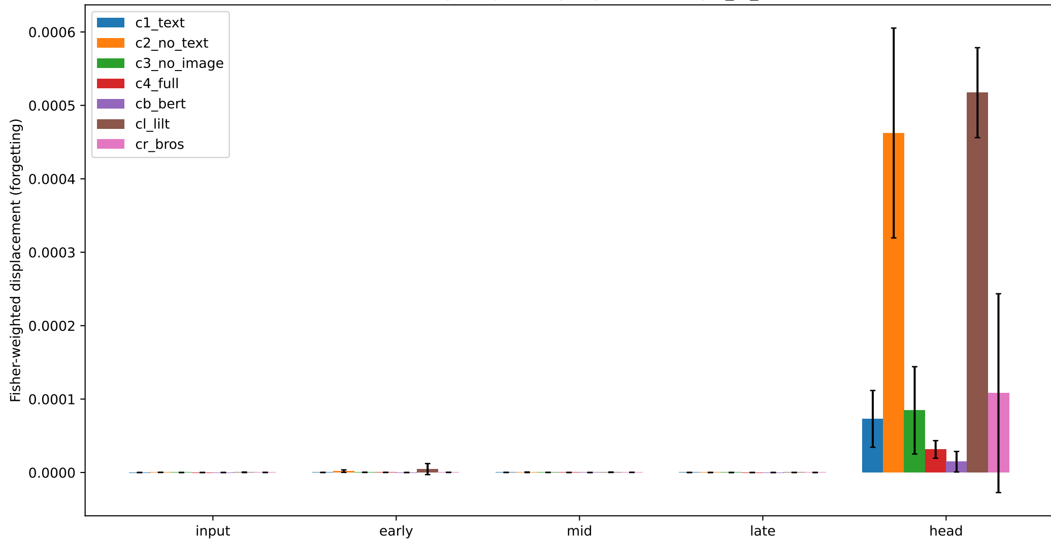
Where forgetting lives by depth (boundary 0_to_1)
