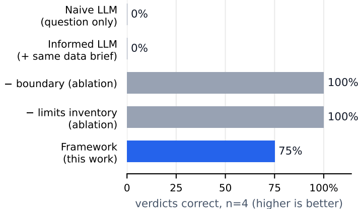
(f) infeasible questions
