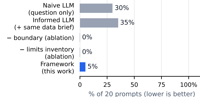
(d) feasibility verdicts that over-claim
