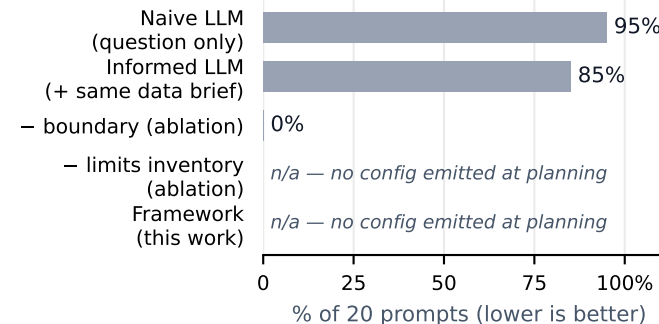
(c) invalid runnable configs
