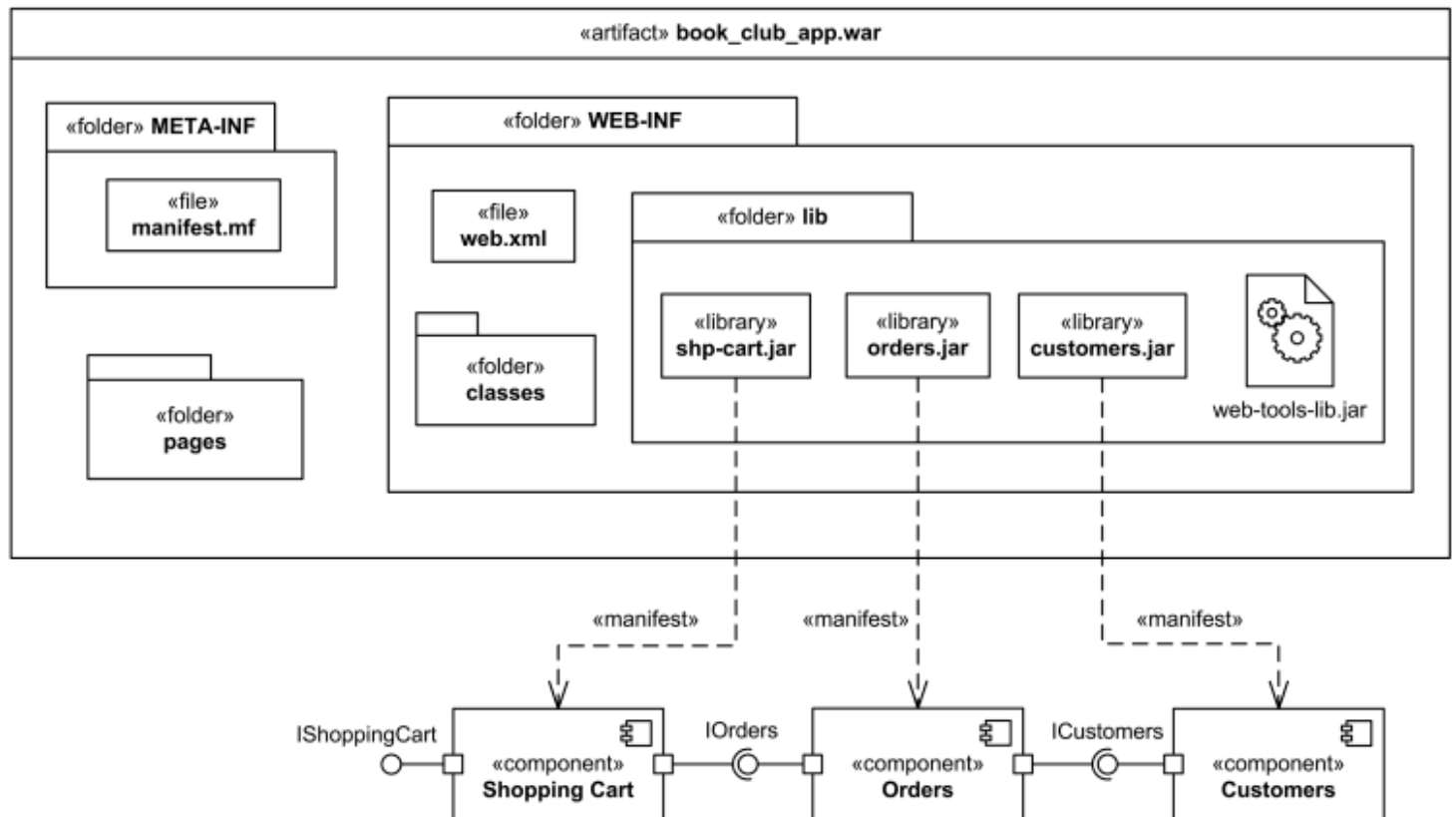
Example of manifestation diagram for web application.
