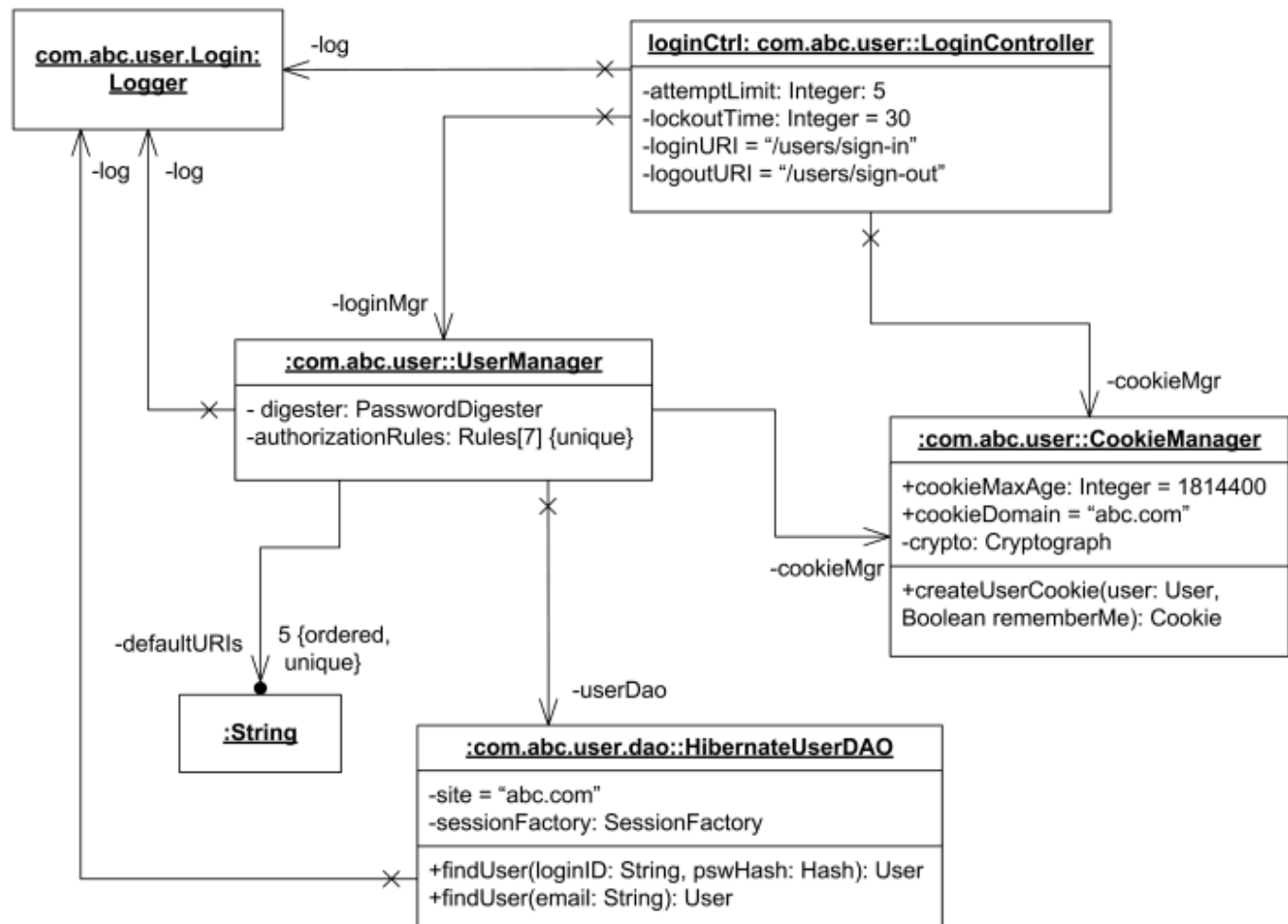
Login Controller object diagram.
