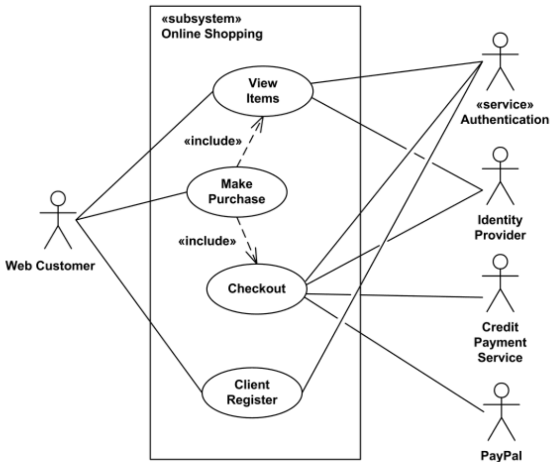
Online Shopping - Top Level Use Cases
