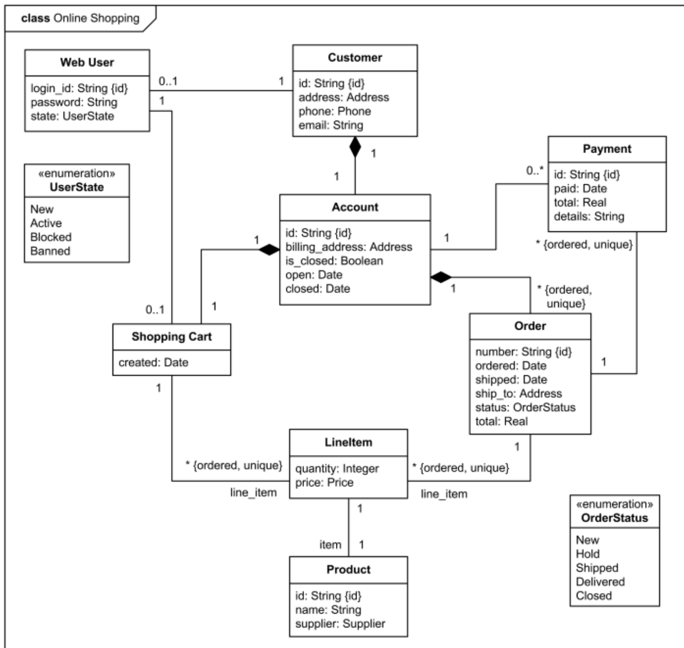
Class diagram example - Online Shopping Domain.
