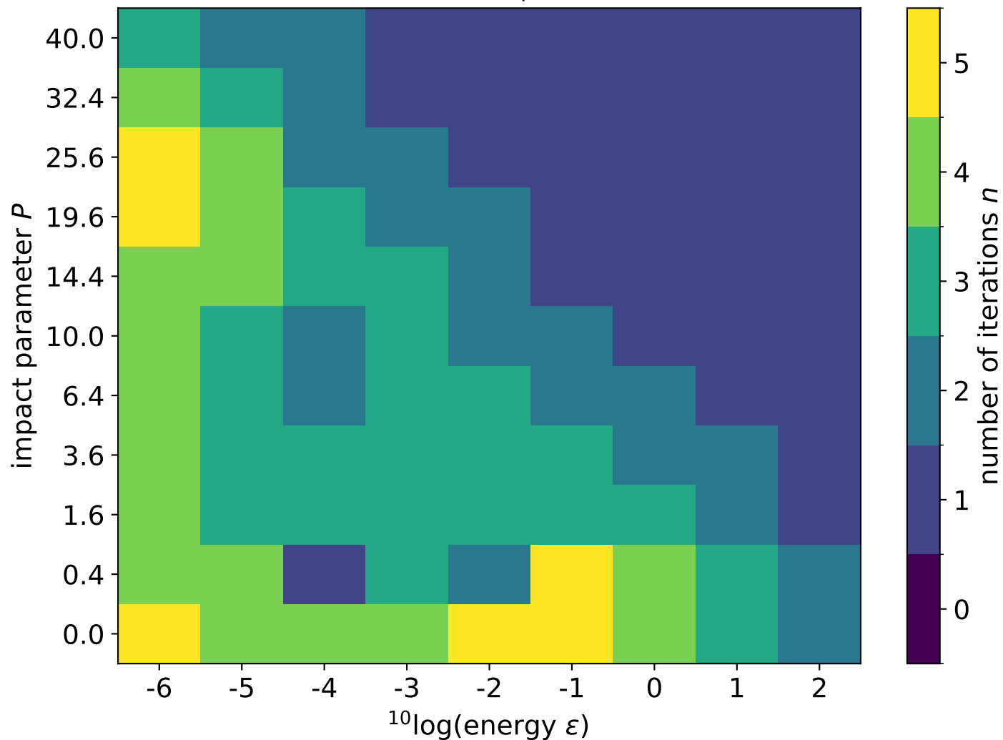
Universal ZBL potential
