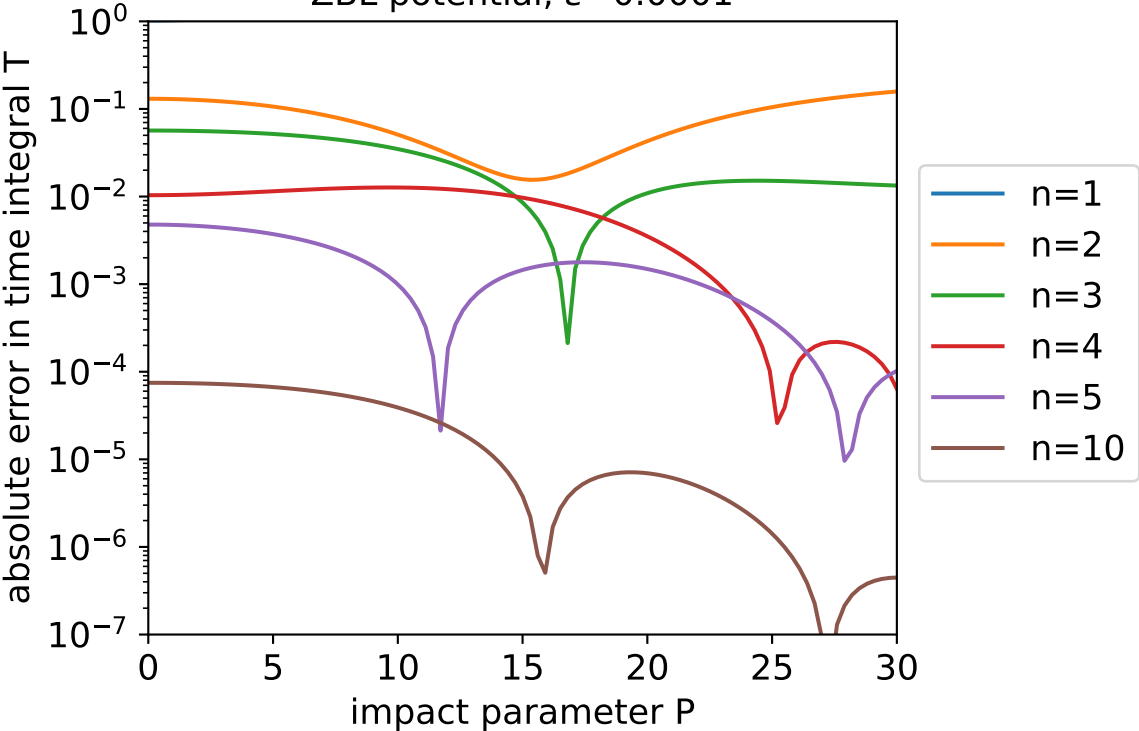
ZBL potential, \varepsilon=0.0001
