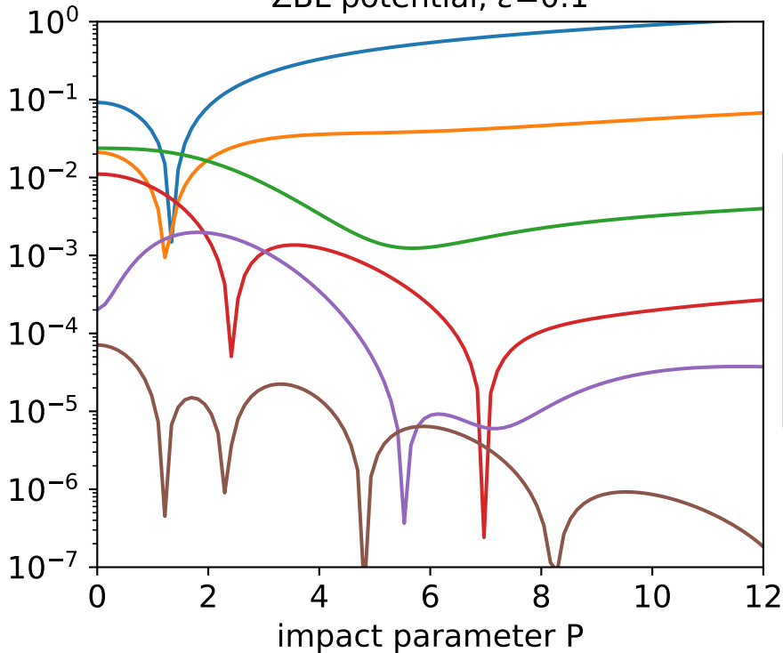
ZBL potential, \varepsilon=0.1
