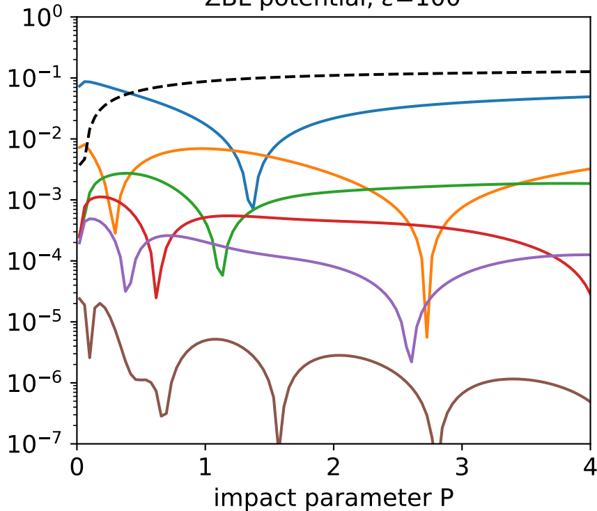
ZBL potential, \varepsilon=100
