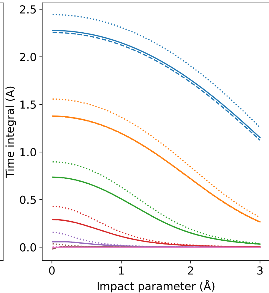
ZBL potential, Z_1=Z_2=14
