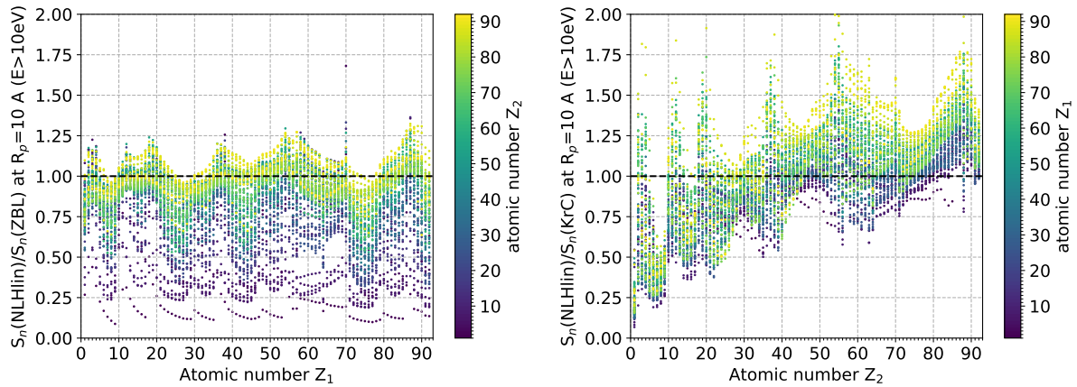
Figure 1.15: Ratio of nuclear stopping cross sections for all atom pair using the NLHlin potential and the ZBL potential (left) of KrC potential (right) at energies that lead to a projected range of 10 Å, but at least 10 eV.
