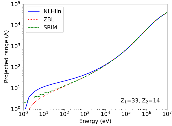
Figure 1.16: Projected range R_p as a function of energy for the NLHlin potential (solid line) and the ZBL potential (dashed and dotted lines). For the ZBL potential, our own results (dotted line) agree well with those obtained by SRIM [11].
