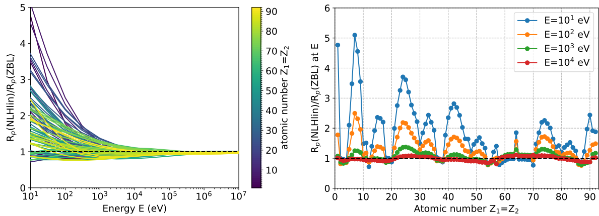
Figure 1.17: The ratio of the projected ranges calculated with the NLHlin and ZBL potentials as a function of energy (left) and as a function of atomic number (right) for homonuclear atom pairs.
