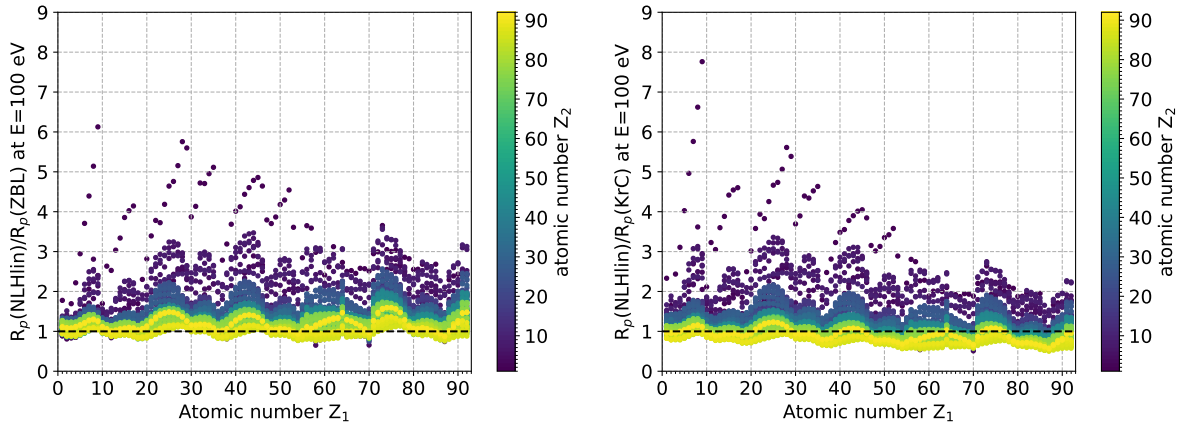
Figure 1.19: Projected range ratio with respect to ZBL (left) and KrC (right) for all combinations of Z_1 and Z_2 .
