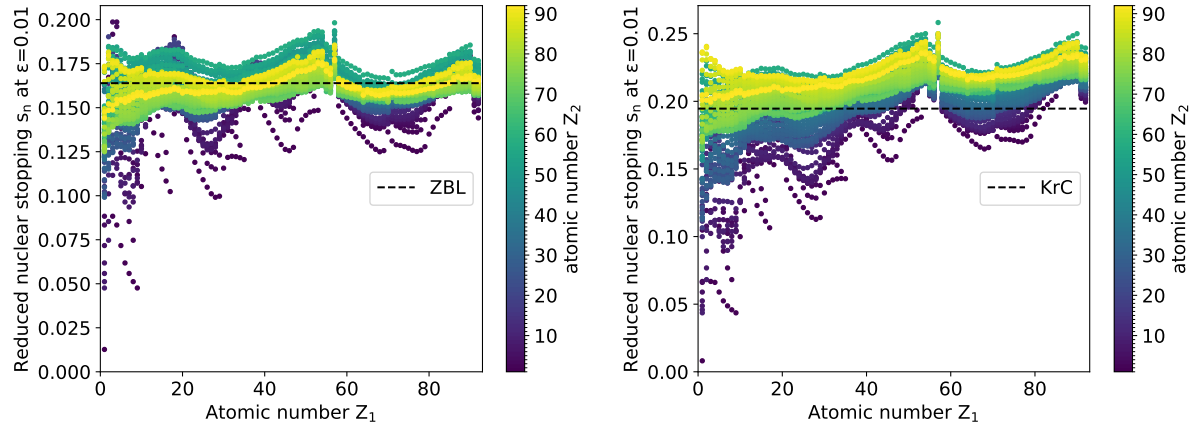
Figure 1.11: Reduced nuclear stopping cross section for the NLHlin potential of all atom pairs as a function of atomic number Z_1 at a reduced energy of \varepsilon = 0.01 . Two different screening lengths have been used. Left: ZBL screening length Eq. (1.13); right: Firsov screening length Eq. (1.11). For comparison, the stopping cross sections of the ZBL potential (left) and the KrC potential (right) are depicted by black dashed lines. Note that these two potentials yield universal reduced stopping cross sections with the respective screening lengths. The atomic numbers Z_2 are color-coded.
