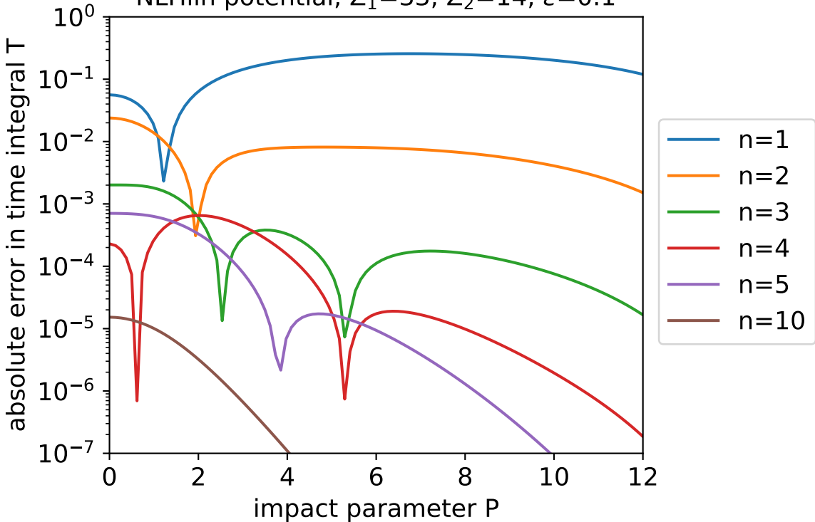
NLHlin potential, Z_1=33 , Z_2=14 , \varepsilon=0.1
