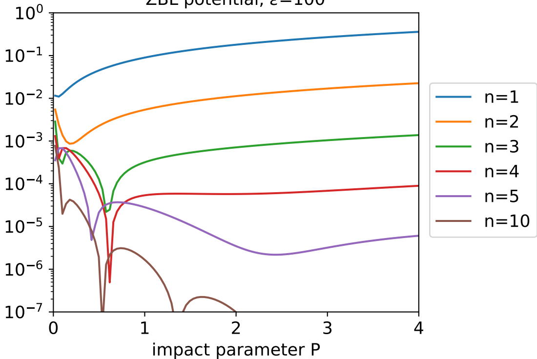
ZBL potential, \varepsilon=100
