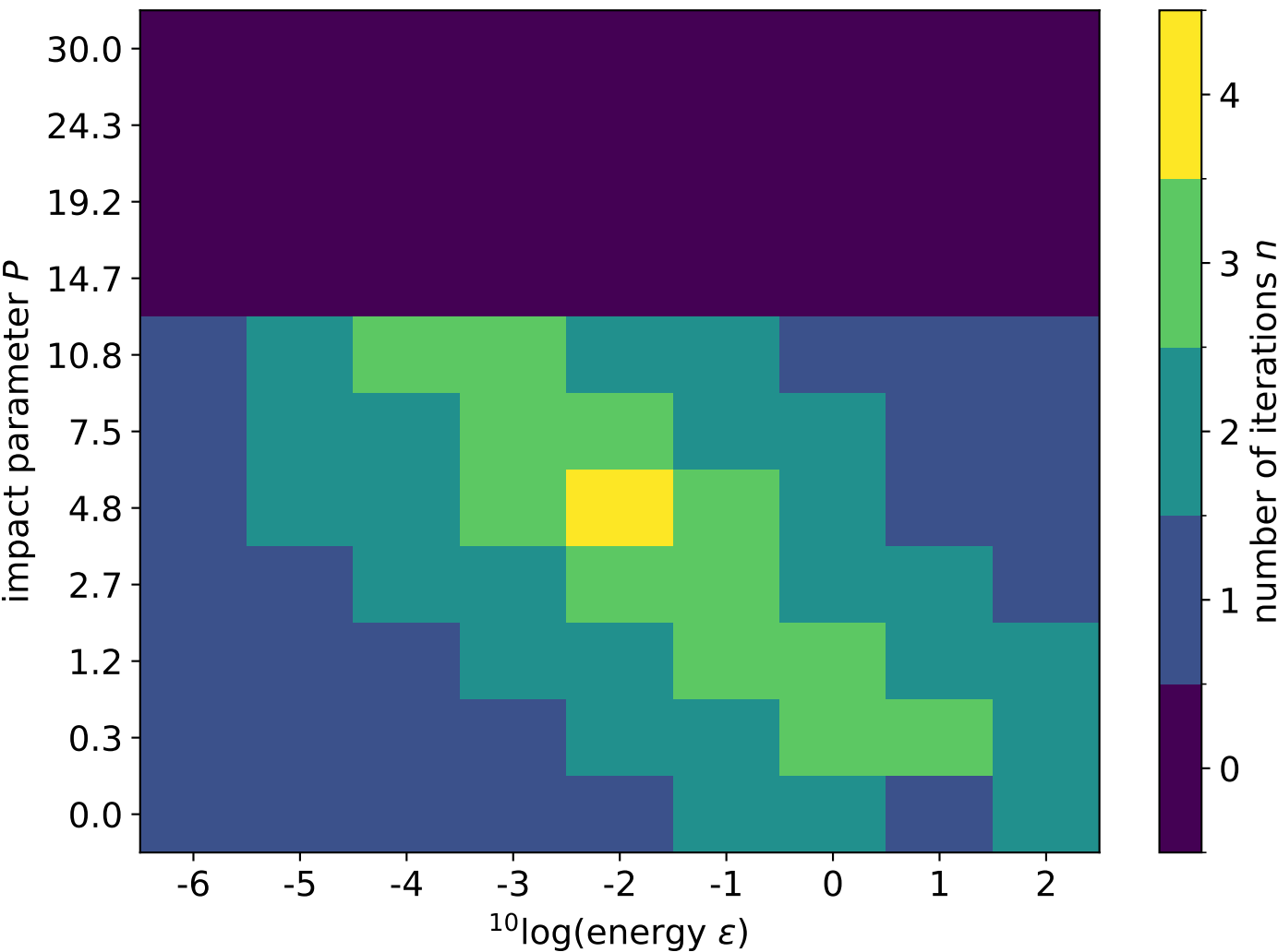
NLHlin potential, Z_1=33 , Z_2=14
