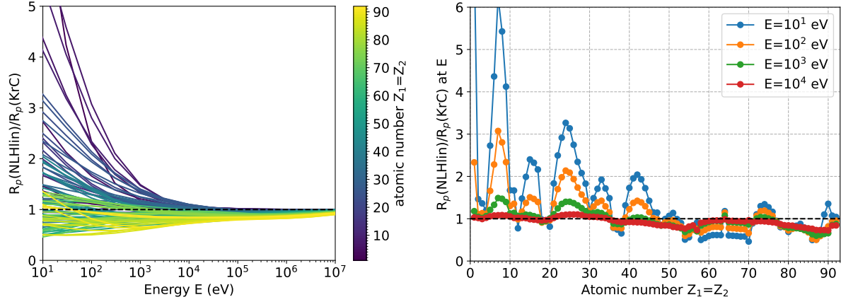
Figure 1.17: The ratio of the projected ranges calculated with the NLHlin and KrC potentials as a function of energy (left) and as a function of atomic number (right) for homonuclear atom pairs.
