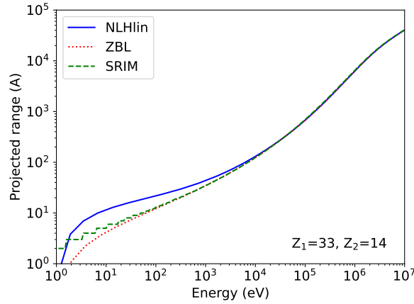
Figure 1.15: Projected range R_p as a function of energy for the NLHlin potential (solid line) and the ZBL potential (dashed and dotted lines). For the ZBL potential, our own results (dotted line) agree well with those obtained by SRIM [11].
