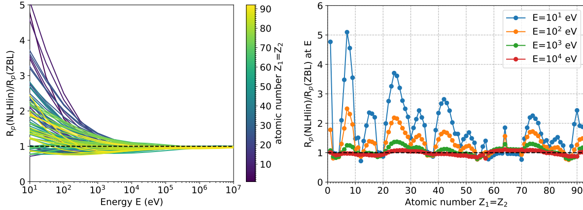
Figure 1.16: The ratio of the projected ranges calculated with the NLHlin and ZBL potentials as a function of energy (left) and as a function of atomic number (right) for homonuclear atom pairs.
