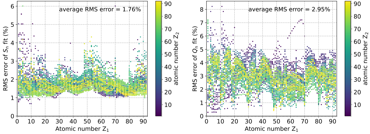
Figure 1.14: Root-mean-square fit errors of the nuclear stopping cross section (left) and nuclear straggling (right) for all atom pairs.
