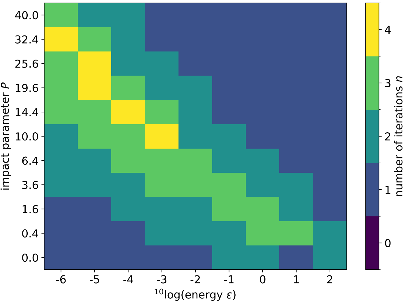
Universal ZBL potential
