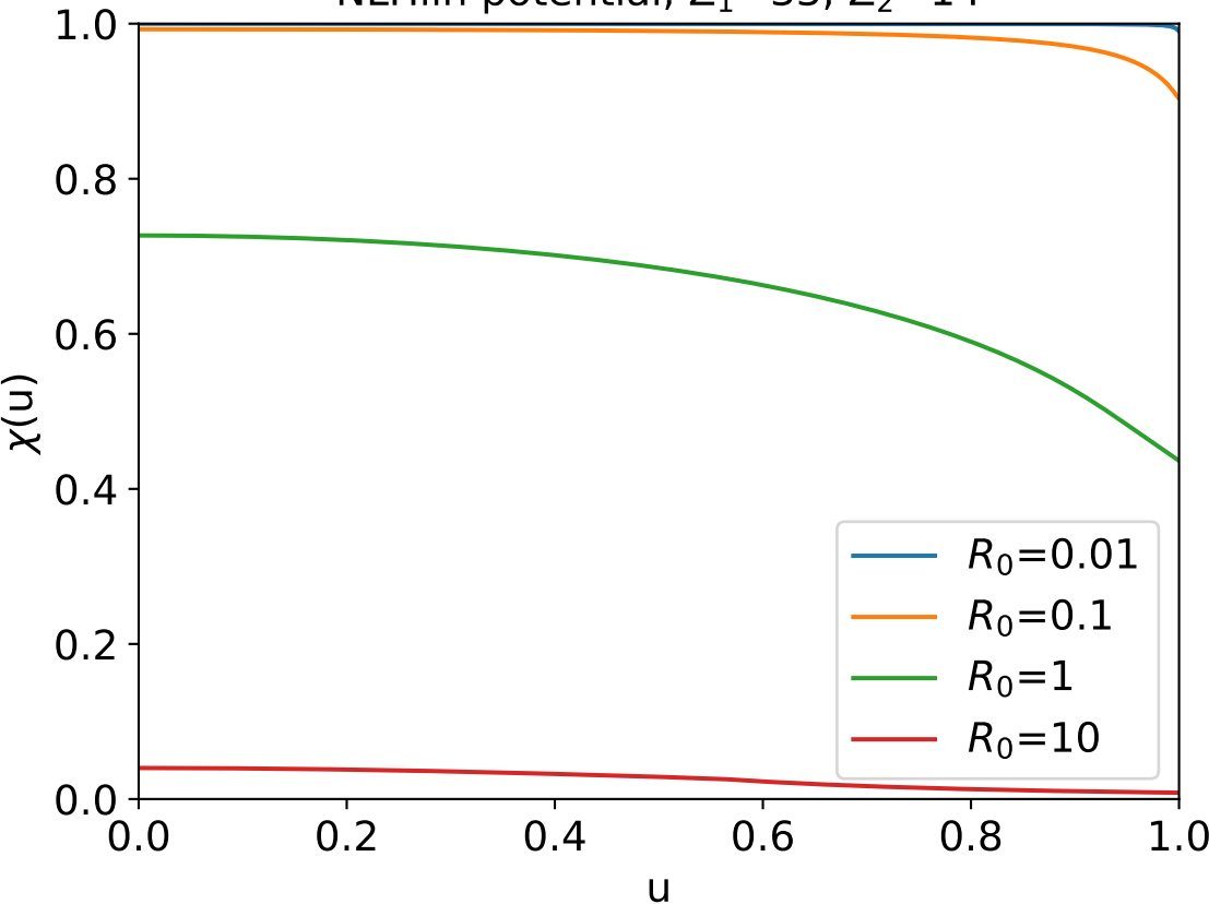
NLHlin potential, Z_1=33 , Z_2=14
