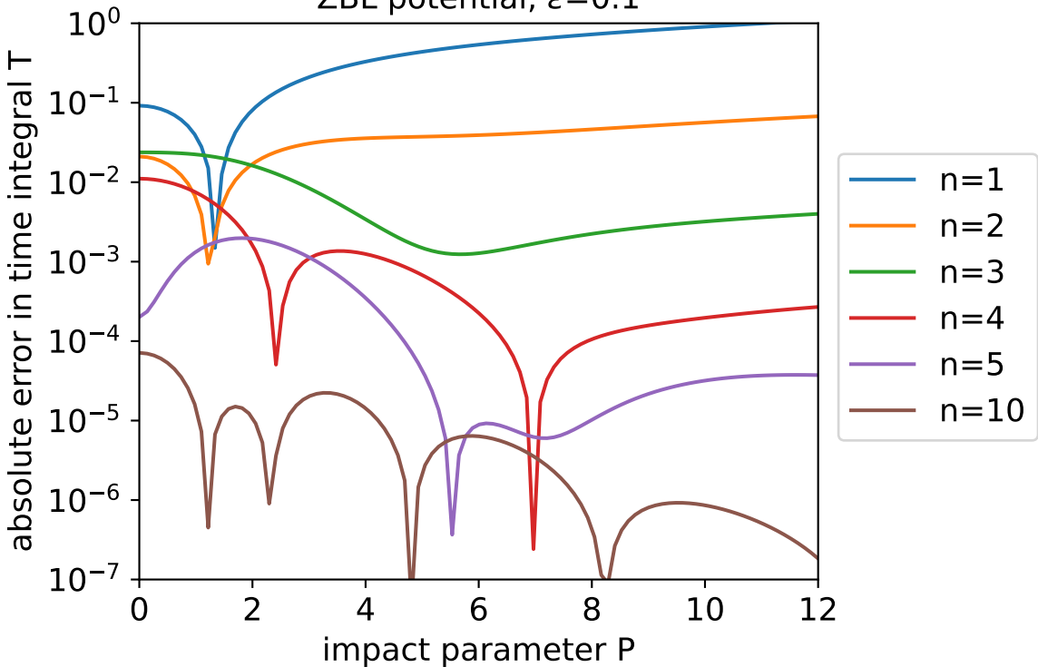
ZBL potential, \varepsilon=0.1
