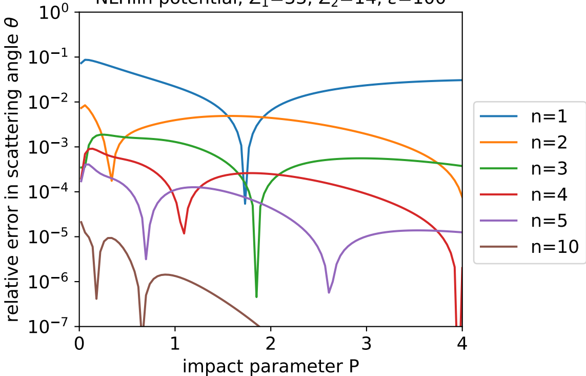
NLHlin potential, Z_1=33 , Z_2=14 , \varepsilon=100
