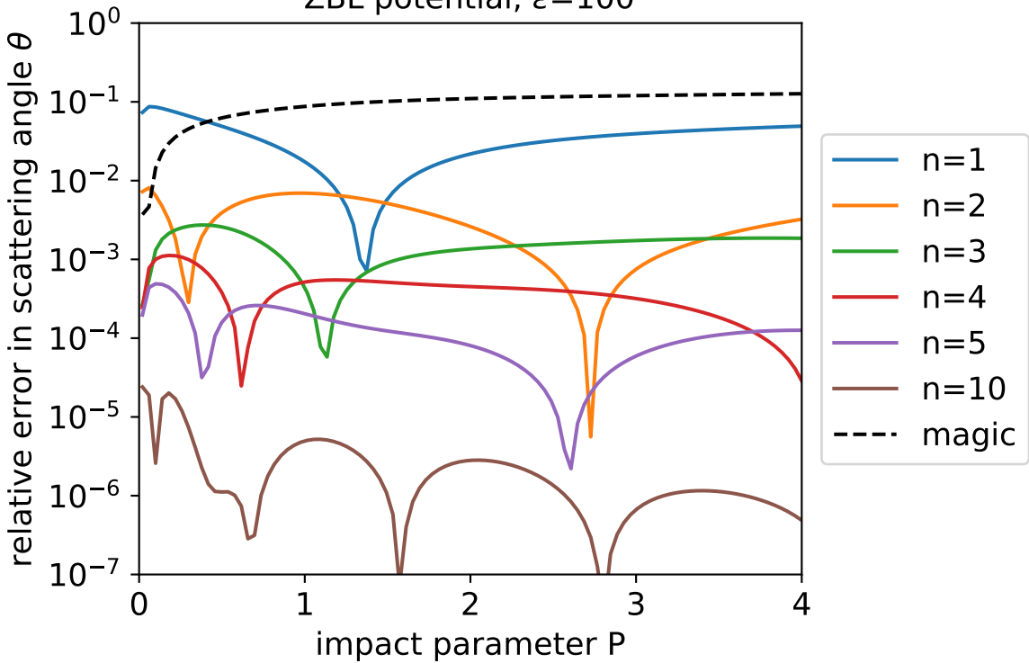
ZBL potential, \varepsilon=100
