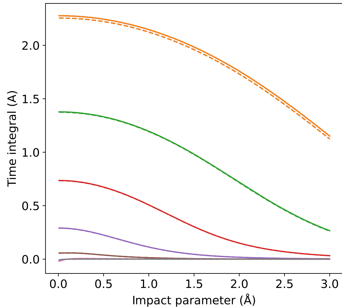
ZBL potential, Z_1=Z_2=14
