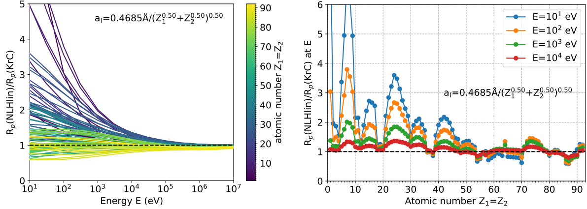
Figure 1.16: The ratio of the projected ranges calculated with the NLHlin and KrC potentials as a function of energy (left) and as a function of atomic number (right) for homonuclear atom pairs.
