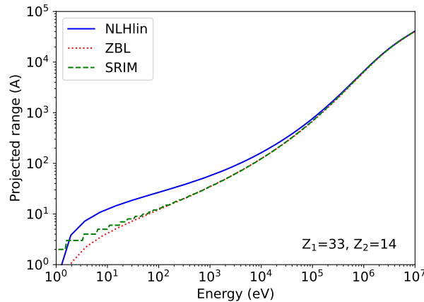
Figure 1.14: Projected range R_p as a function of energy for the NLHlin potential (solid line) and the ZBL potential (dashed and dotted lines). For the ZBL potential, our own results (dotted line) agree well with those obtained by SRIM [11].
