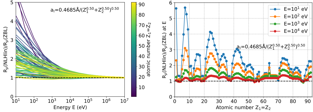
Figure 1.15: The ratio of the projected ranges calculated with the NLHlin and ZBL potentials as a function of energy (left) and as a function of atomic number (right) for homonuclear atom pairs.
