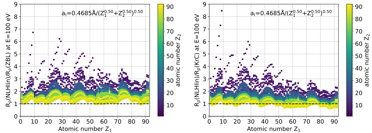
Figure 1.17: Projected range ratio with respect to ZBL (left) and KrC (right) for all combinations of Z_1 and Z_2 .
