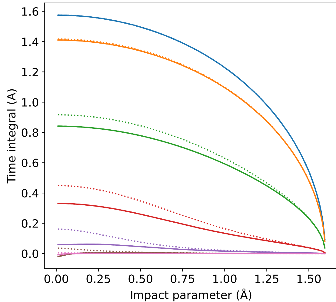
NLHlin potential, Z1=Z2=14
