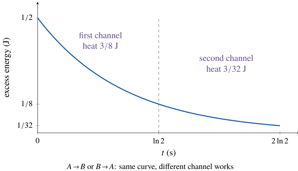
Figure 5. Exact excess-energy decay during two finite charge-sharing stages. The continuous state is the same for both orders, while the channel receiving the larger heat transfer changes. The plotted curve is equation (45).
