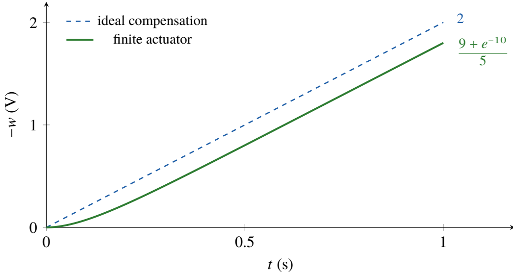
Figure 4. Exact reference-cell response from equation (37), with C = 1 F, a = 2 V/s, and \tau_a = 1/10 s. The plotted quantities are the stated closed forms, with their exact one-second endpoints.
