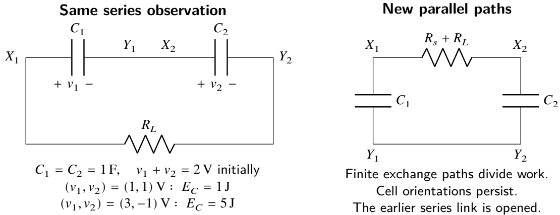
Figure 8. Two equal series cells can have the same terminal voltage and different internal energy. A later parallel connection exposes the difference mode only through its declared finite paths; the individual cell orientations remain fixed.
