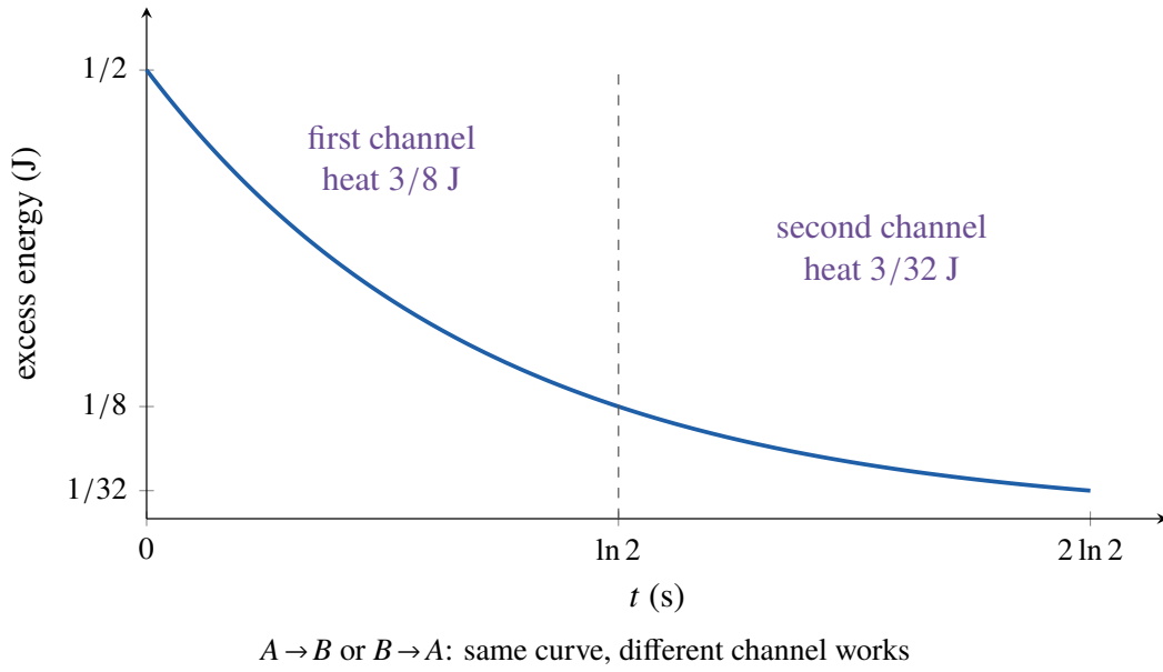
Figure 9. Exact excess-energy decay during two finite charge-sharing stages. The continuous state is the same for both orders, while the channel receiving the larger heat transfer changes. The plotted curve is equation (94).
