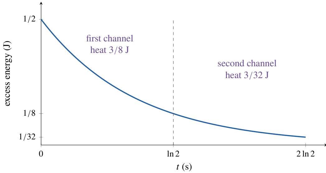
Figure 8. Exact excess-energy decay during two finite charge-sharing stages. The continuous state is the same for both orders, while the channel receiving the larger heat transfer changes. The plotted curve is equation (71).
