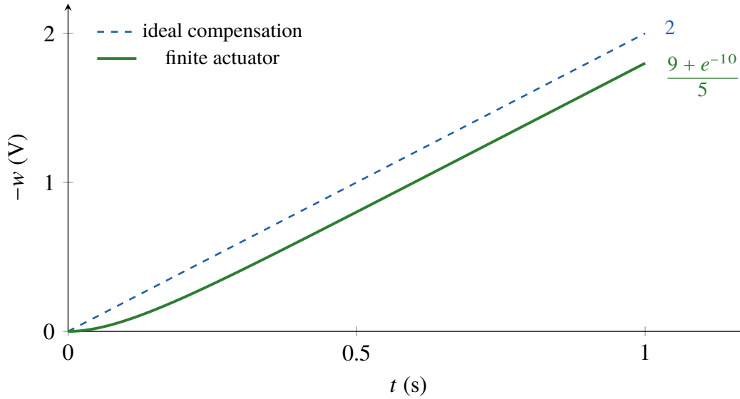
Figure 5. Exact reference-cell response from equation (46), with C = 1 F, a = 2 V/s, and \tau_a = 1/10 s. The plotted quantities are the stated closed forms, with their exact one-second endpoints.
