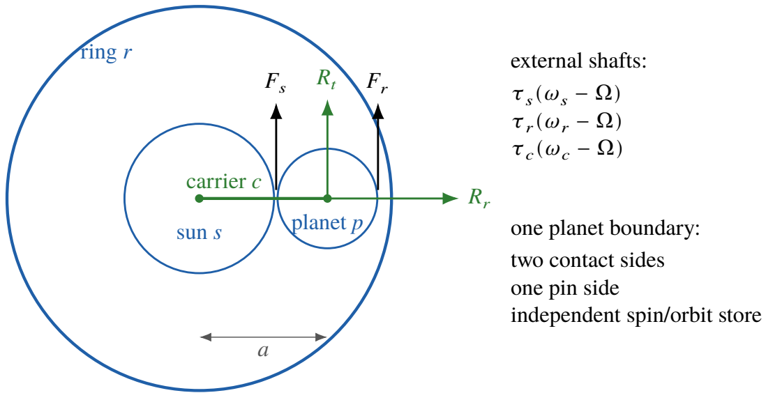
Figure 2. Schematic pitch contacts and external shaft ports. Only one planet is drawn. Force arrows indicate positive tangential and radial components; their signed values follow the free bodies.
