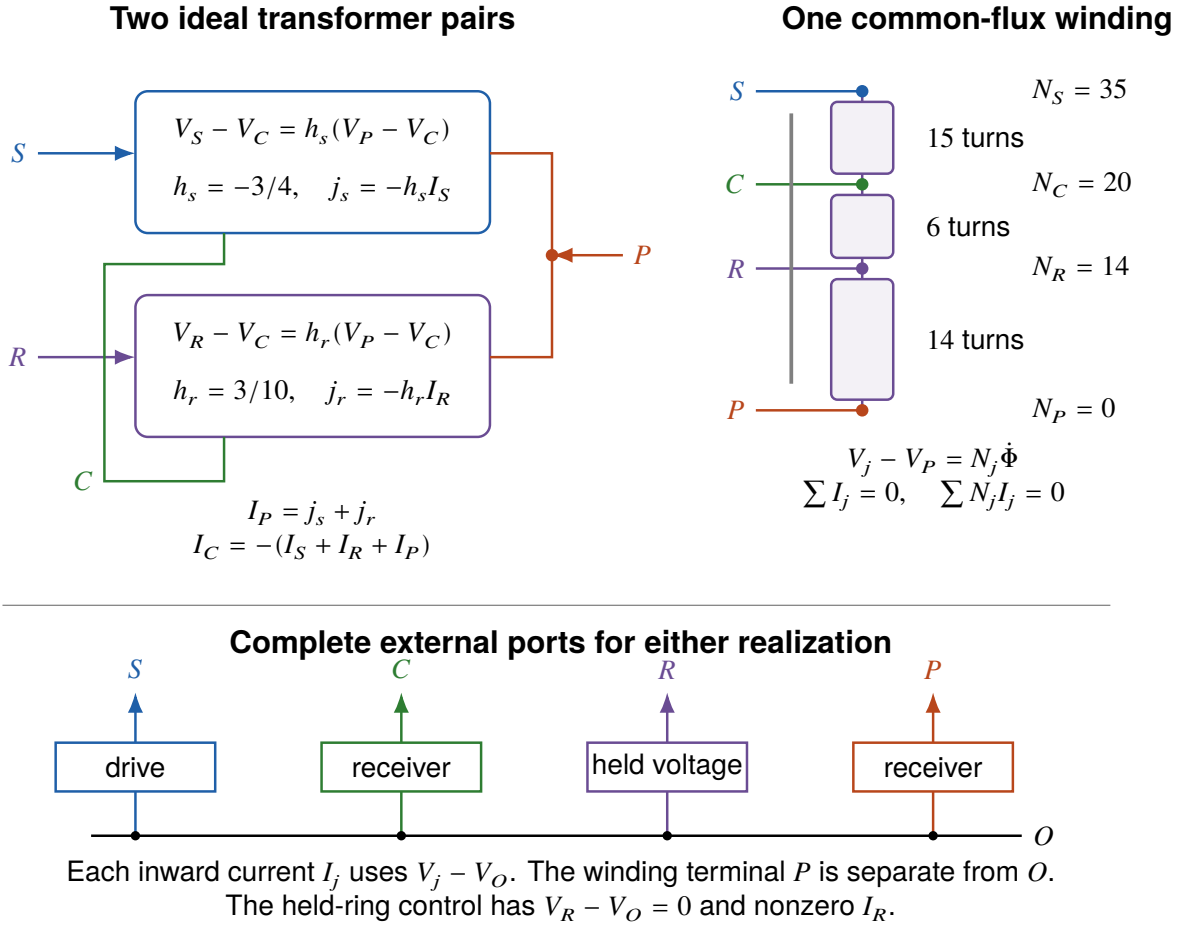
Figure 4. Two ideal realizations of the same four-terminal relation. Left: signed sun and ring transformer ratios with their secondary currents entering the planet node. Right: four taps on one common-flux winding; numbers are cumulative turns from P. Each external port is a terminal-to-O connection. P is loaded, and O is an external physical return separate from the winding.
