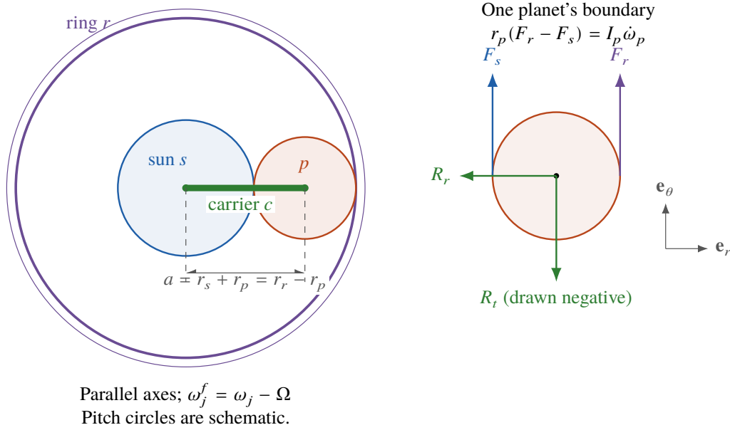
Figure 2. Schematic pitch geometry and forces on one planet. Blue identifies the sun, orange the planet, green the carrier, and purple the ring. Tangential mesh forces on the planet have signed components F_s, F_r ; its pin force is R_t \mathbf{e}_\theta + R_r \mathbf{e}_r . Only one of the three planets is drawn.
