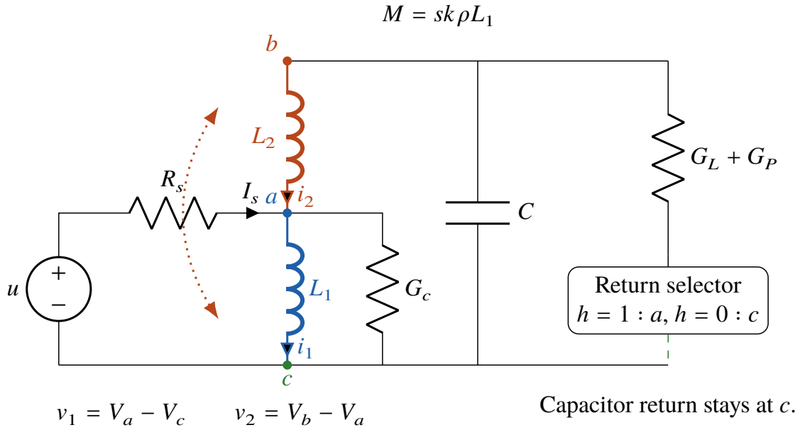
Figure 3. Schematic tapped circuit. The source reaches a through R_s ; the coupled winding sections are a-c and b-a . The capacitor remains across b-c . The receiver and probe may return to a or c , while the effective core-loss conductance remains across a-c . Dotted coupling is magnetic, not a wire.
