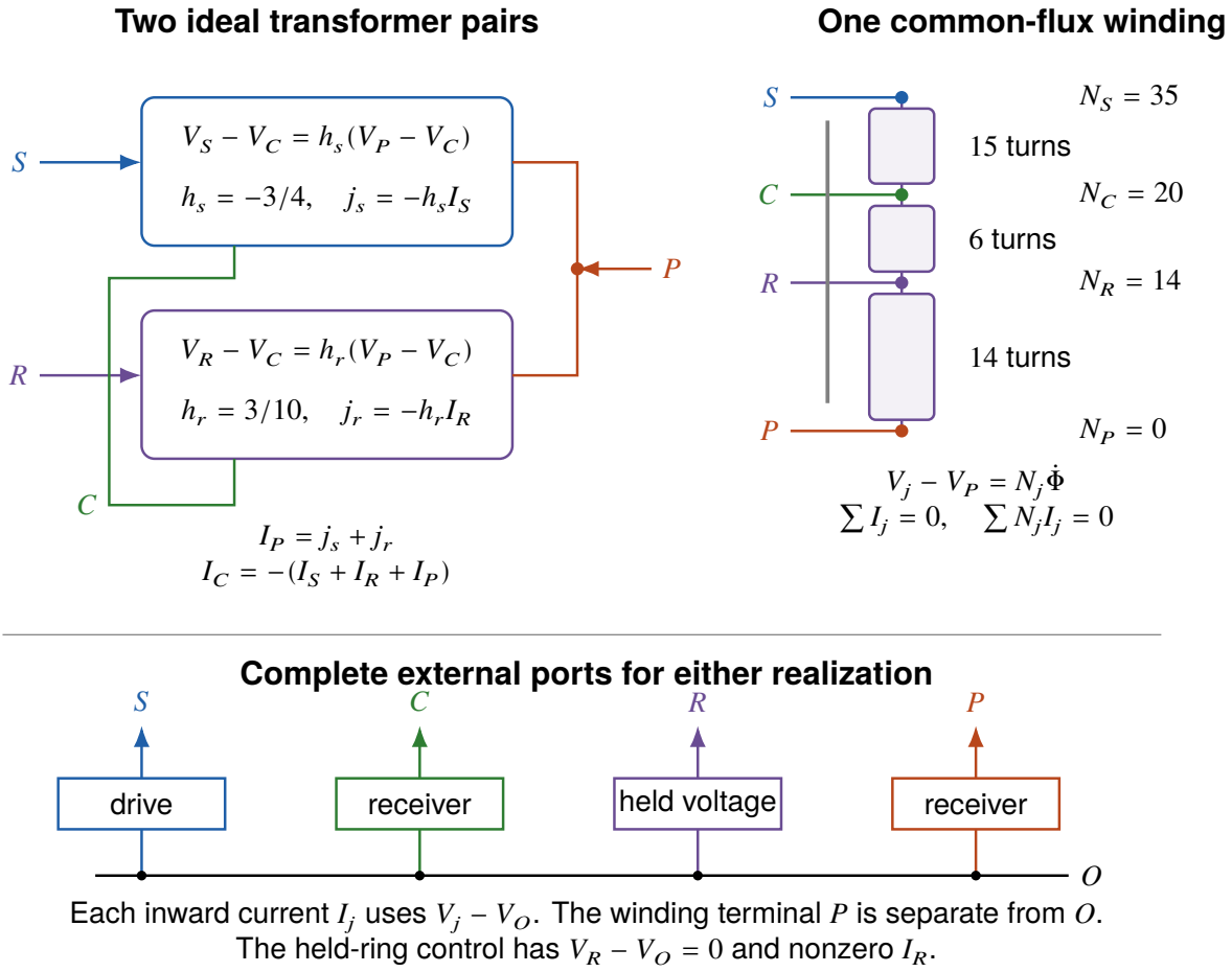
Figure 3. Two ideal realizations of the same four-terminal relation. Left: signed sun and ring transformer ratios with their secondary currents entering the planet node. Right: four taps on one common-flux winding; numbers are cumulative turns from P. Each external port is a terminal-to-O connection. P is loaded, and O is an external physical return separate from the winding.
