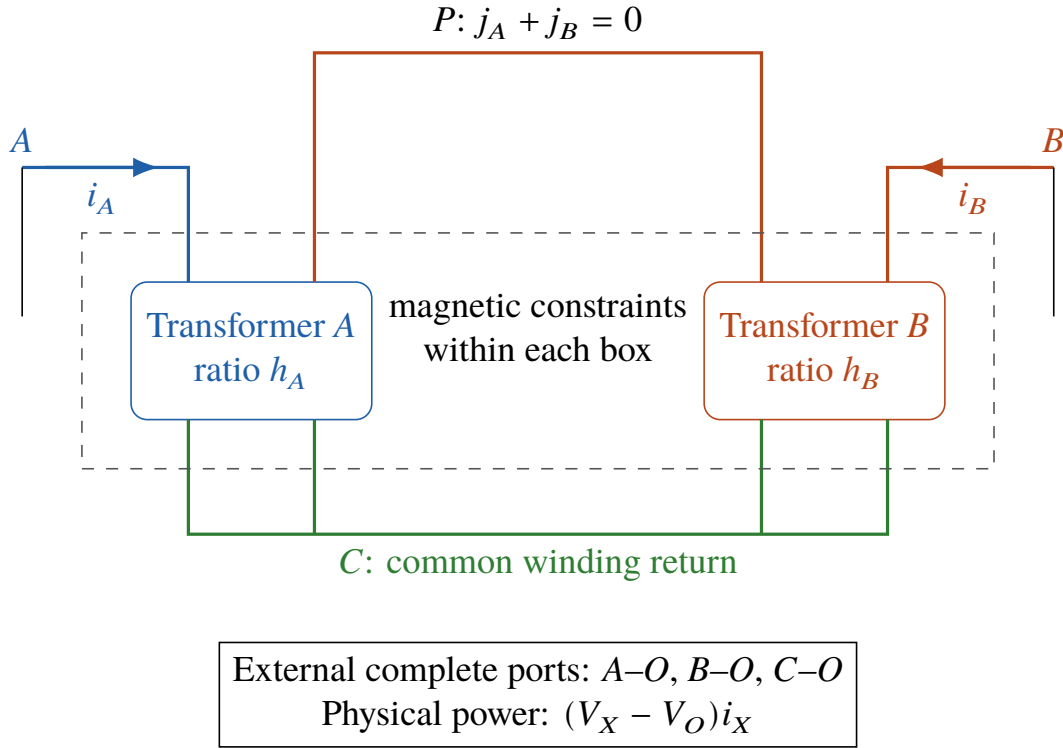
Figure 8. Schematic two-transformer compound correspondence. Both secondary windings share P – C ; the complete external ports connect A, B, C to the physical return O . The four winding ports are internal to the complete network. A common shift of all node potentials, including O , preserves every complete port voltage.
