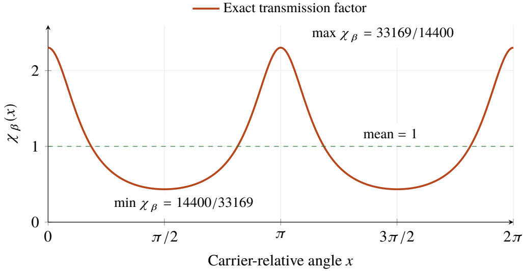
Figure 4. Exact quarter-turn Hooke transmission factor from equation (56), with \cos^2 \beta = 14400/33169 . The ripple is periodic in the carrier-relative input angle. Its mean is one even though the instantaneous factor ranges between the annotated exact bounds. The illustrative articulation is not asserted to be practical.
