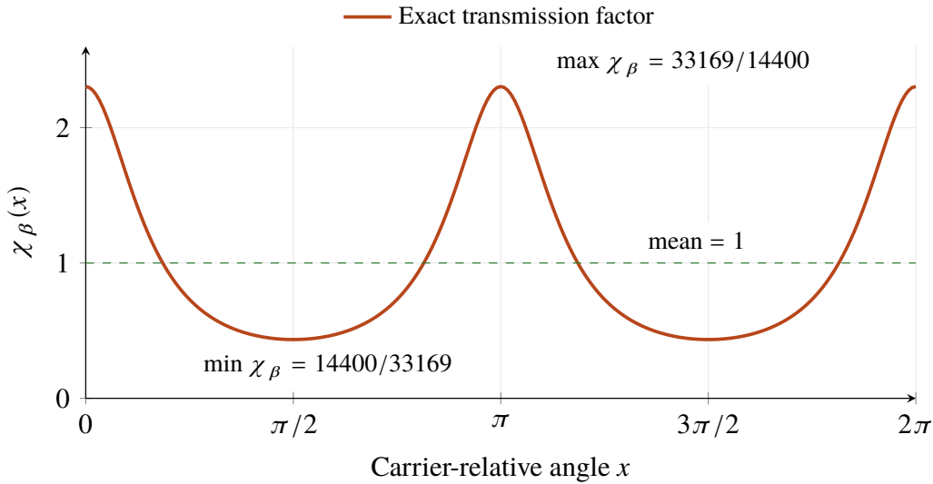
Figure 4. Exact quarter-turn Hooke transmission factor from equation (29), with \cos^2 \beta = 14400/33169 . The ripple is periodic in the carrier-relative input angle. Its mean is one even though the instantaneous factor ranges between the annotated exact bounds. The illustrative articulation is not asserted to be practical.
