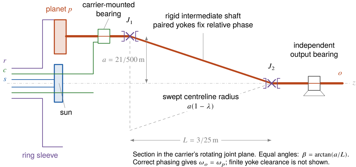
Figure 1. Schematic four-shaft construction, shown in a carrier-dependent axial plane. Separate sun, carrier and ring sleeves terminate before the illustrated joint sweep; their connections continue to their respective gear members. The planet stub rotates in a carrier-mounted bearing. Crosses and paired yoke marks show the two joints and the relative phasing fixed by the intermediate shaft. Dashed lines bound the swept centreline; real yokes, shaft radii, bearing loads and collision clearances require a separate design.
