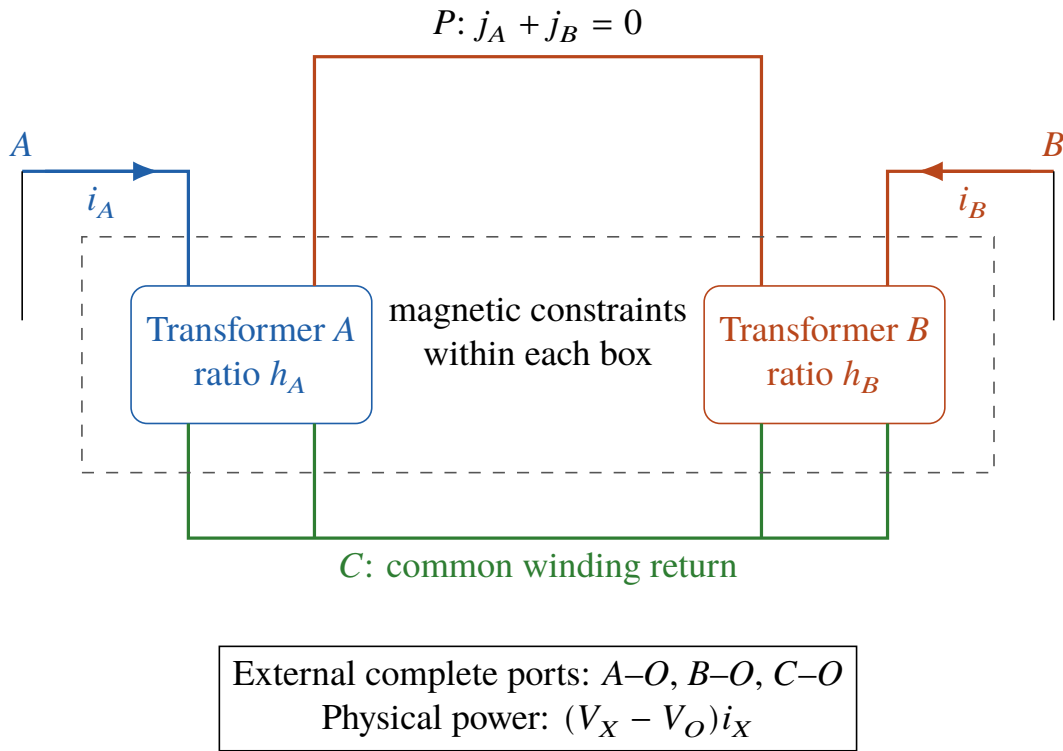
Figure 8. Schematic two-transformer compound correspondence. Both secondary windings share P-C ; the complete external ports connect A, B, C to the physical return O . The four winding ports are internal to the complete network. A common shift of all node potentials, including O , preserves every complete port voltage.
