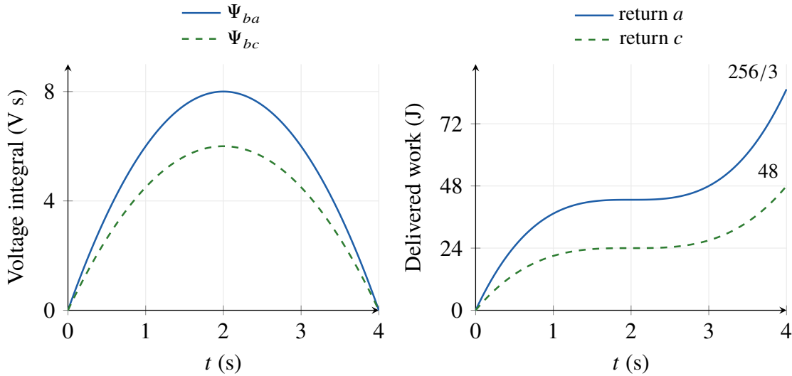
Figure 6. Exact reversing-drive control: the voltage integrals return to zero, while delivered load works increase as the integral of squared voltage. Time is in seconds; the two load connections are distinct ideal experiments driven by the same prescribed v_1 = t - 2 .
