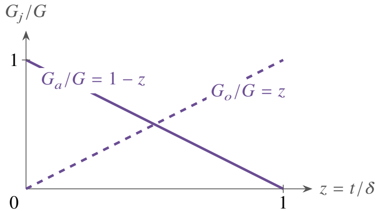
Figure 7. Schematic receiver connections during commutation. Both controlled branches remain distinct; G_a returns to a , while G_o and the fixed capacitor return to c . The source and tapped windings connect to these same terminals as in Figure 5. The lower plot gives the exact bounded overlap history in equation (110).
