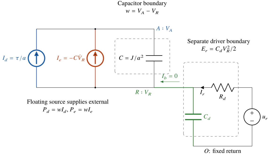
Figure 9. Schematic active reference cell. The two floating sources drive the capacitor between A and R ; their supplies lie outside the capacitor boundary. A separate R_d, C_d driver sets the physical reference potential. The net bias current is zero in this ideal floating cell, while the driver capacitor and resistor still require their own input work.
