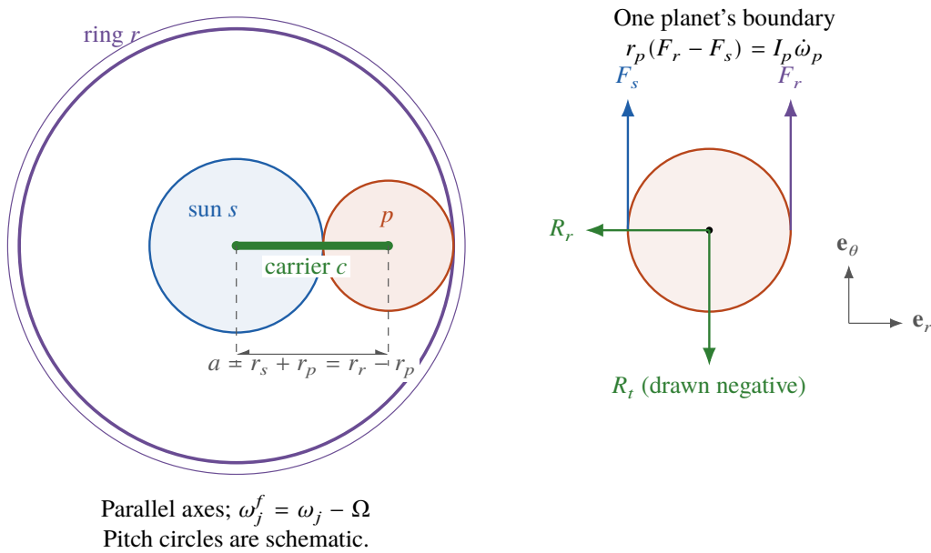
Figure 3. Schematic pitch geometry and forces on one planet. Blue identifies the sun, orange the planet, green the carrier, and purple the ring. Tangential mesh forces on the planet have signed components F_s, F_r ; its pin force is R_t \mathbf{e}_\theta + R_r \mathbf{e}_r . Only one of the three planets is drawn.
