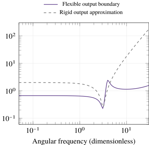
Boundary stiffness magnitude
