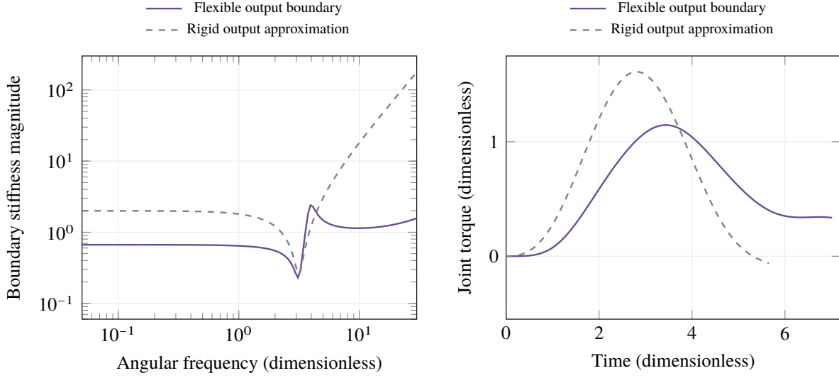
Figure 4. A separate flexible output boundary exposes a resonance and changes joint torque, even when the contact peak is similar. Parameters are those of the declared illustration. Torque curves end at each model's separation; both axes use the dimensionless units of the comparison.
