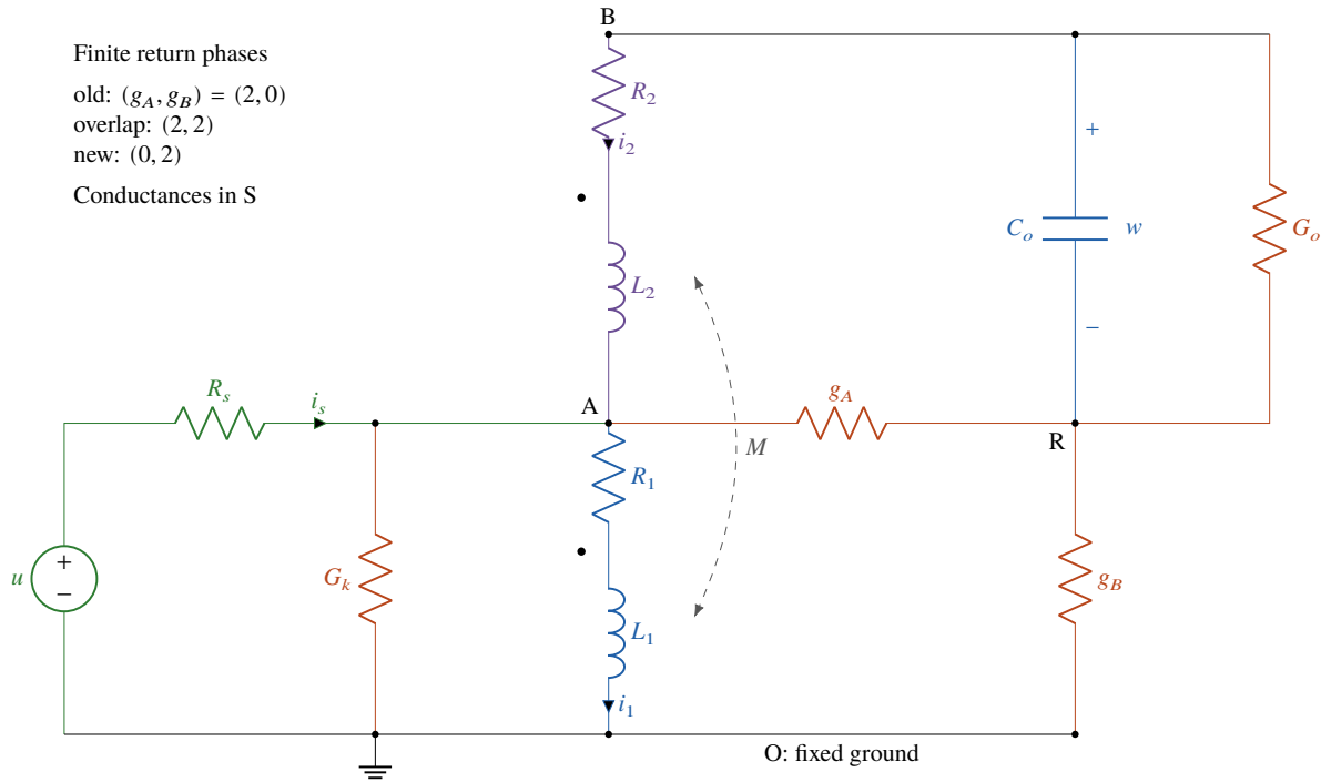
Figure 4. Schematic of the complete return commutation. The two winding sections remain connected and magnetically coupled throughout. The old return is A and the new return is O; their finite conductances overlap. The resistive clamp has its own measured power.
