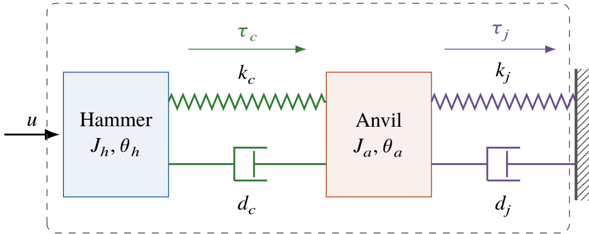
Reactive boundary: two inertias and two springs Damper heat leaves; a moving fixture would add a work port.
