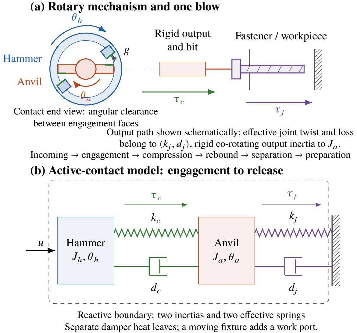
Figure 2. Schematic rotary impact-driver mechanism and its active-contact abstraction. Matching colors identify hammer, anvil and rigid output, deforming contact, and effective joint response. The angular face clearance closes at engagement; the spring-damper laws apply on the indicated contact interval. Separate damper channels export heat from the reactive boundary.
