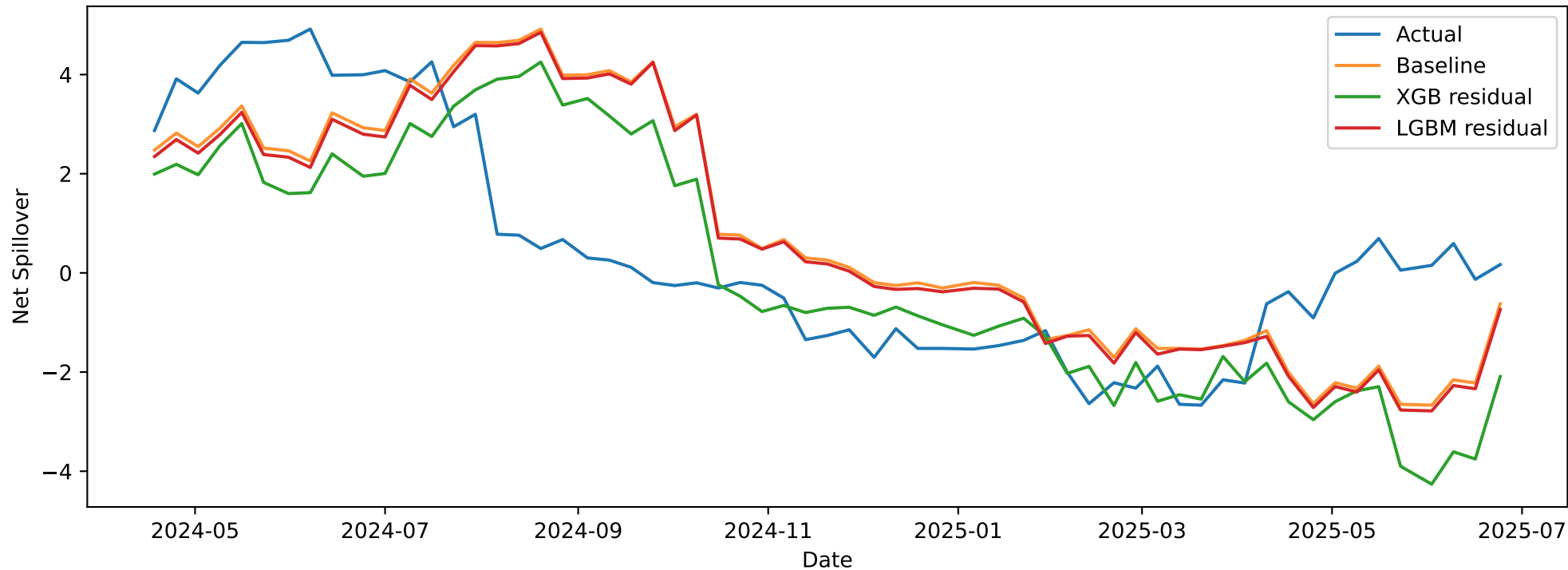
IEF: Walk-forward — Last Fold
