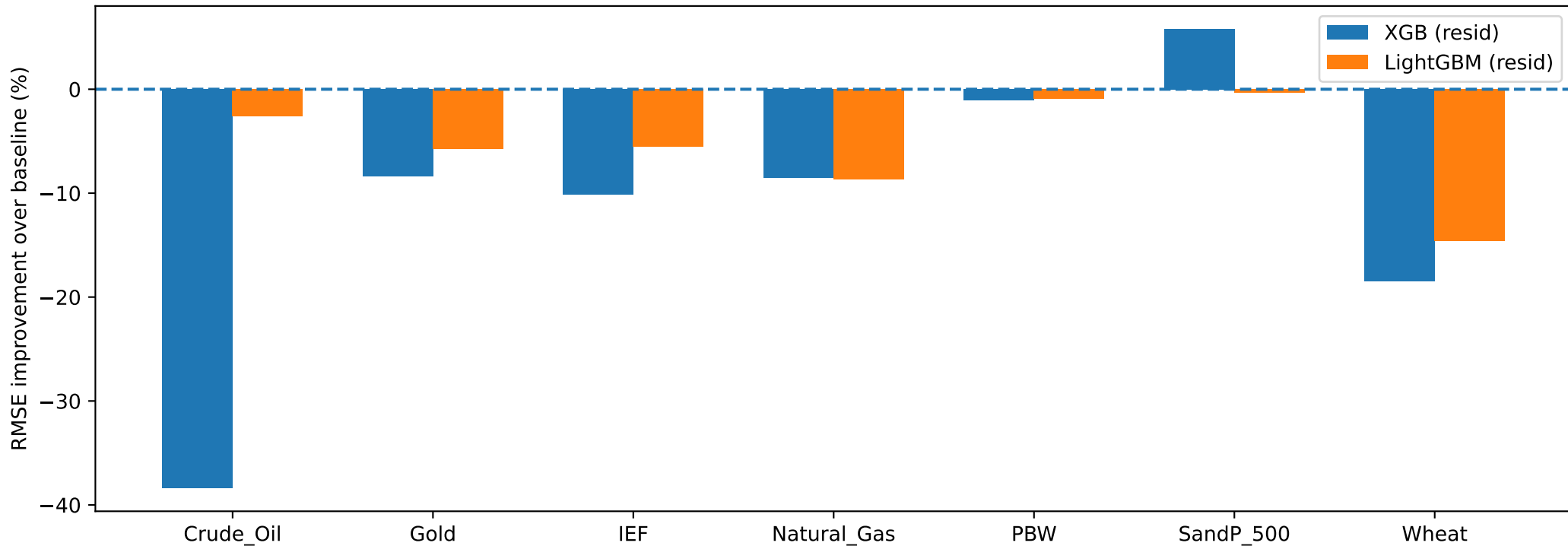
Per-asset: RMSE reduction vs baseline (walk-forward averages)
