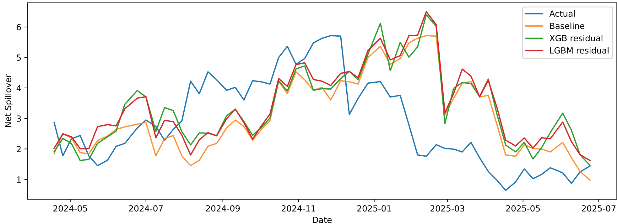
PBW: Walk-forward — Last Fold
