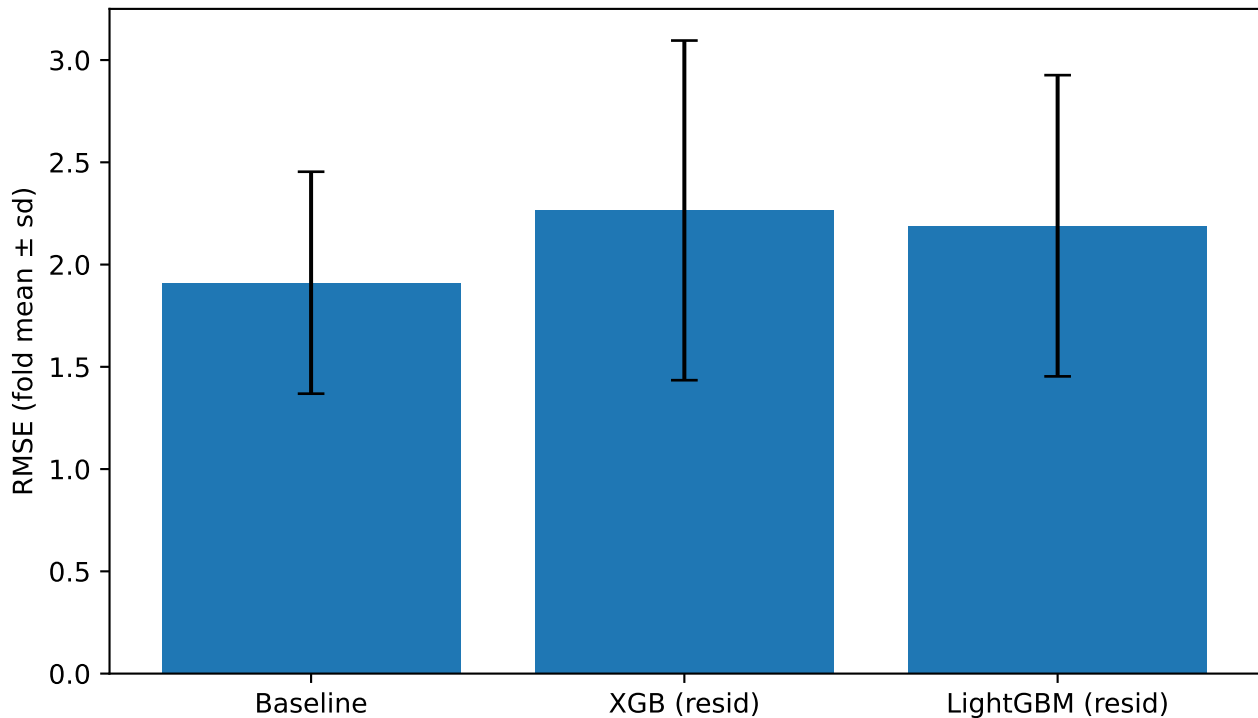
Wheat: Walk-forward RMSE by model
