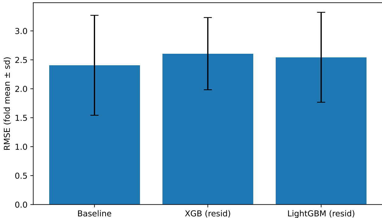
Gold: Walk-forward RMSE by model
