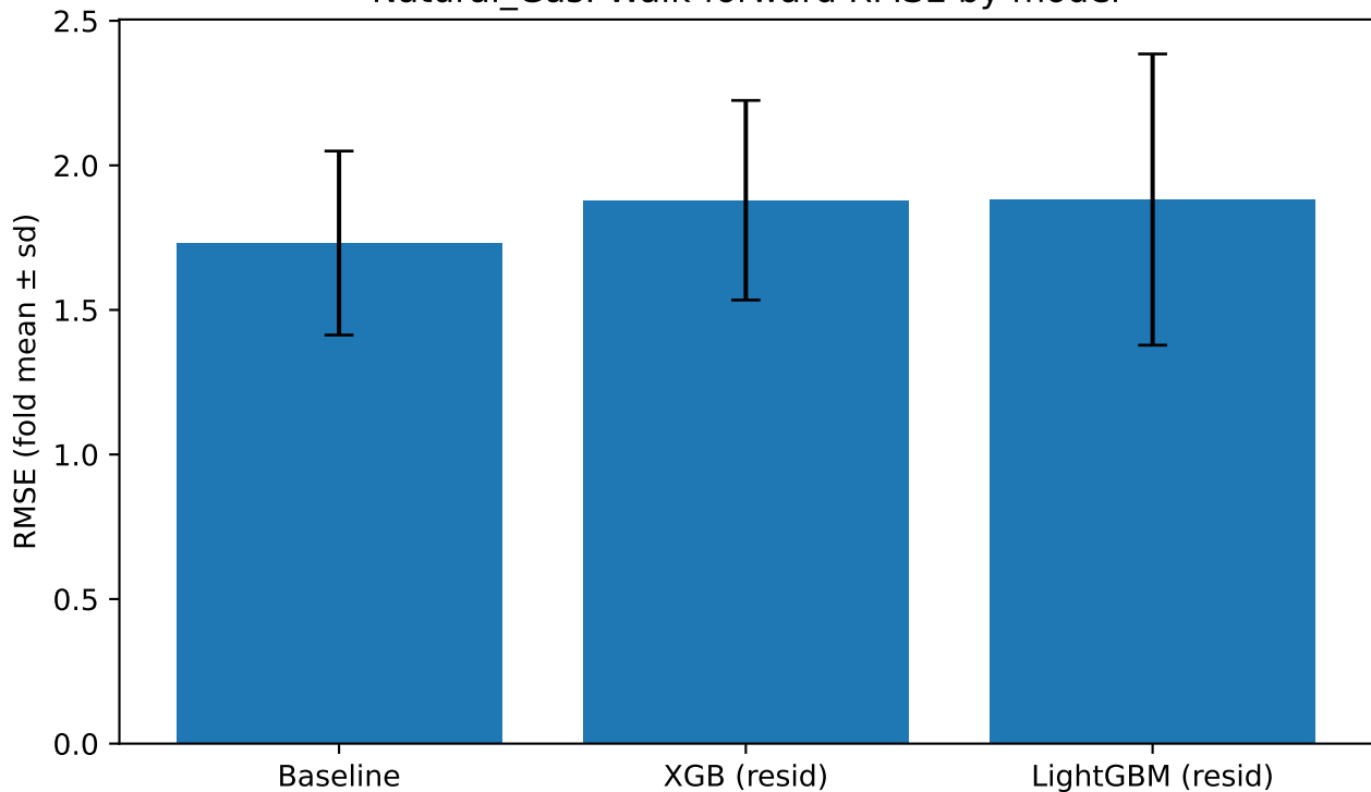
Natural_Gas: Walk-forward RMSE by model
