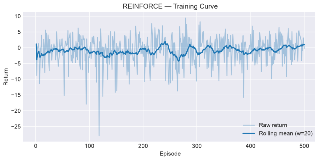
Figure 2. REINFORCE episodic return over 500 episodes. First-50 average: -1.06. Last-50 average: 0.64 (absolute gain +1.70).
