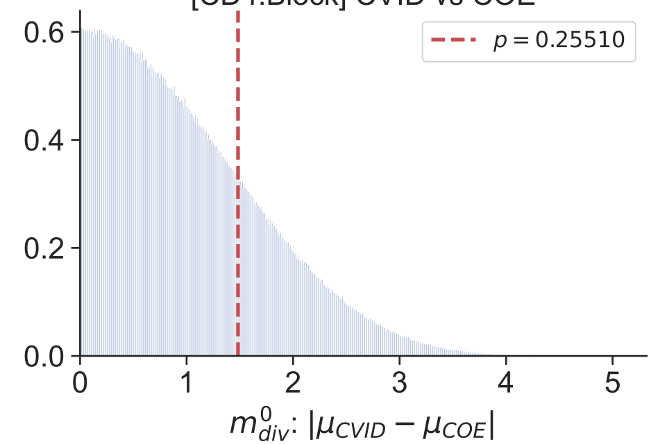
[CD4:Block] CVID vs COE
