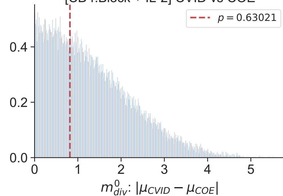
[CD4:Block + IL-2] CVID vs COE
