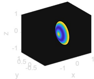
intersection: surface solution at time .10
