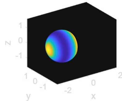
difference: surface solution at time 10
