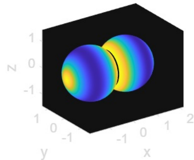
union: surface solution at time 0.
