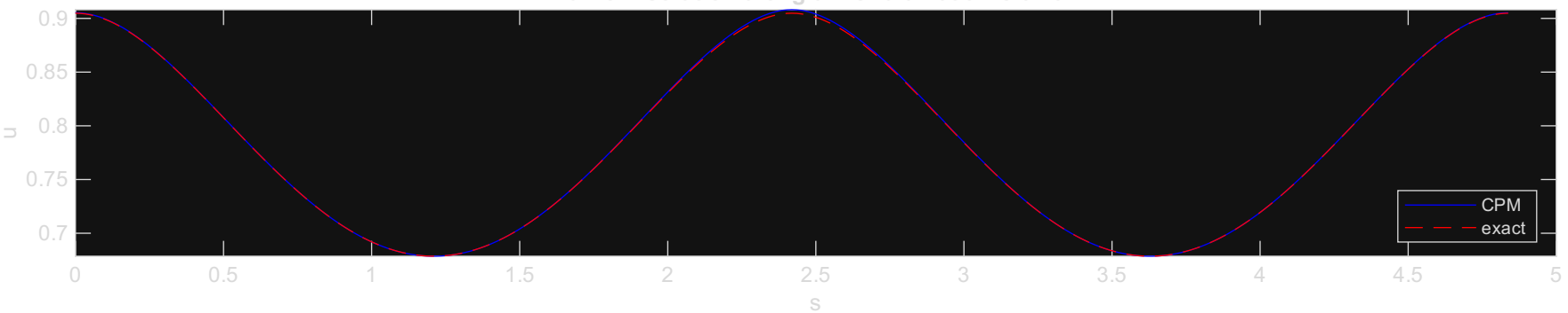
intersection: solution along a meridian at time 0.10
