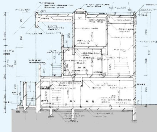
Section Detail 1/100
