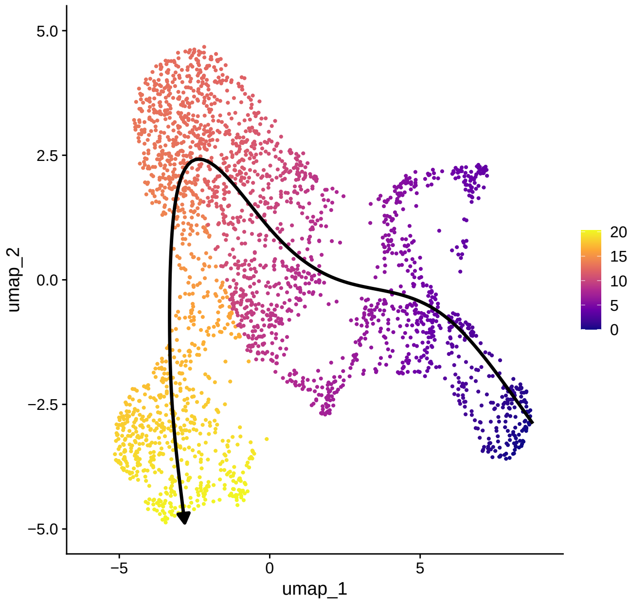
Slingshot_Pseudotime_start_pre_muLEC_lin1
